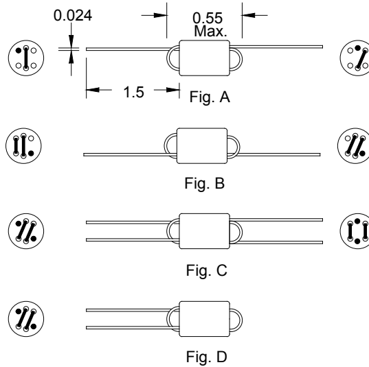
Core Dimension
