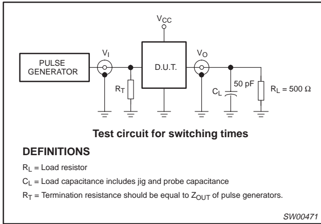
Figure 5. Load circuitry for A outputs
