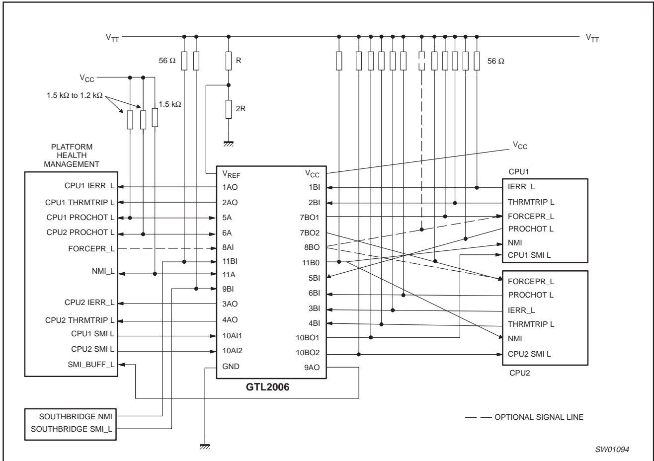
Figure 3. Application diagram
