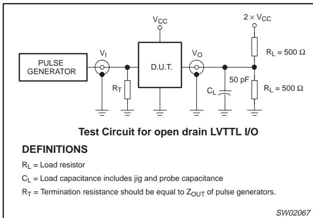
Figure 6. Load circuitry for open drain LVTTL I/O
