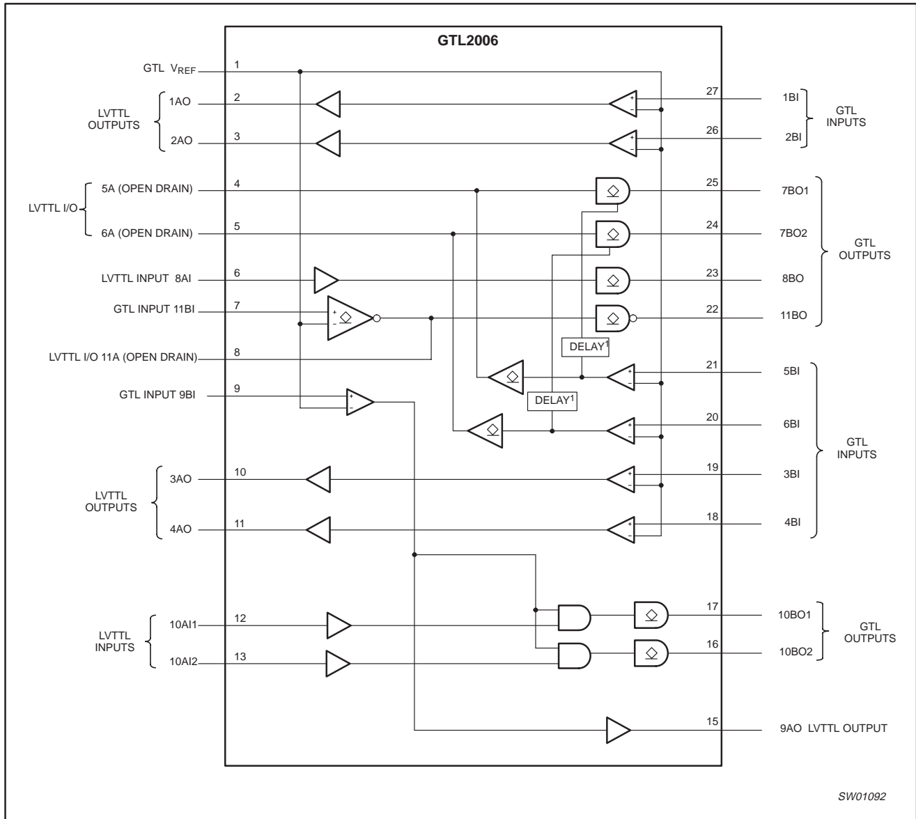
Figure 2. Logic symbol
