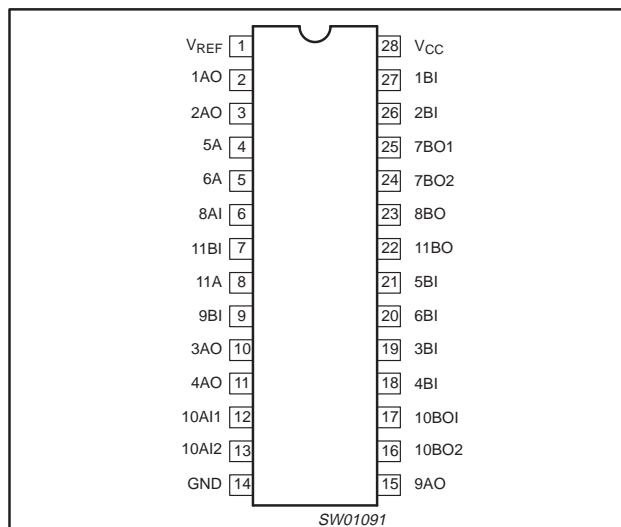
Figure 1. Pin configuration
