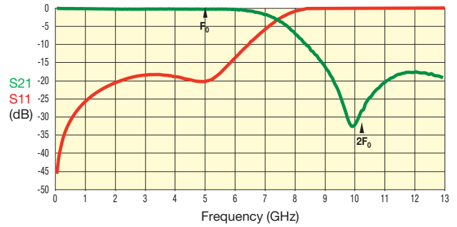
LP0603N5200ANTR
