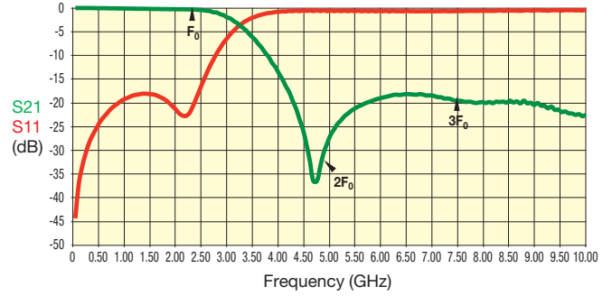
LP0603A2442ANTR
