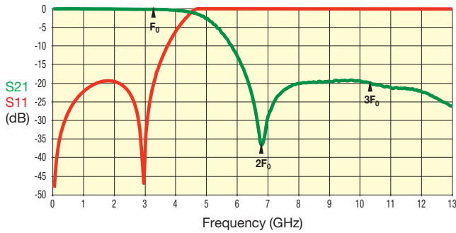
LP0603N3500ANTR
