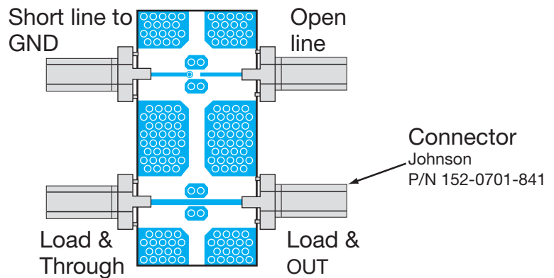
Calibration Jig
