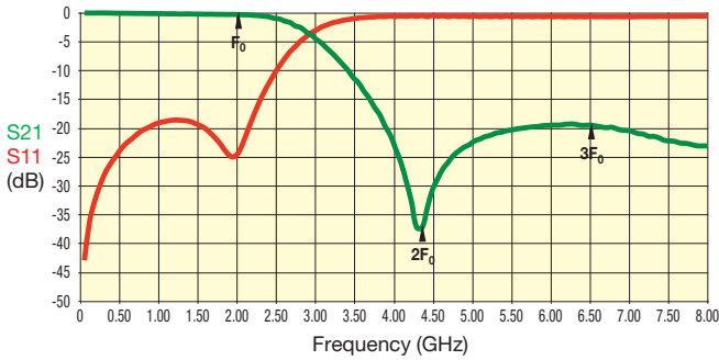
LP0603A2140ANTR
