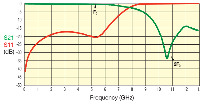
LP0603N5500ANTR
