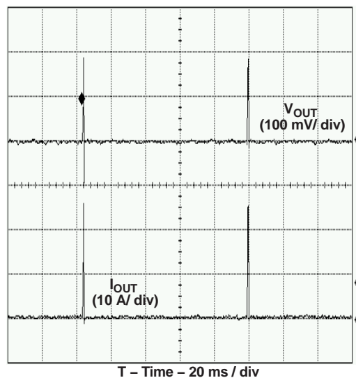
Figure 2. Output Fault Hiccup Restart Timing
