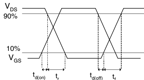
Fig 17. Switching Time Waveforms
