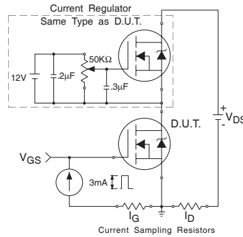
Fig 15. Gate Charge Test Circuit
