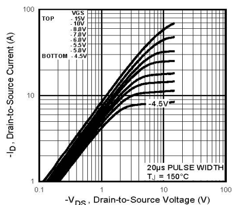
Fig 13. Typical Output Characteristics, T_J = 150^\circ C
