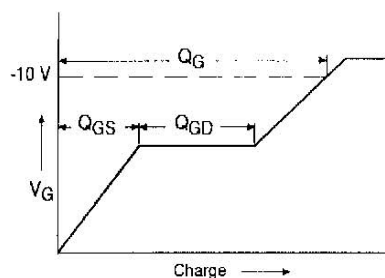
Fig 22b. Basic Gate Charge Waveform
