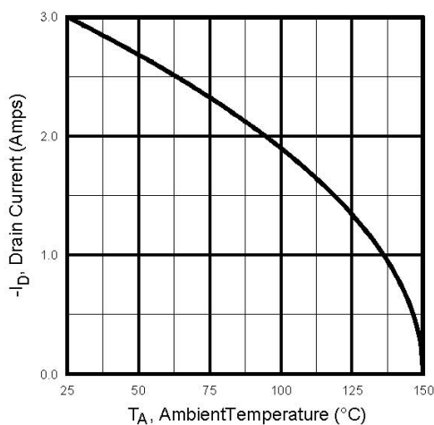
Fig 20. Max. Drain Current Vs. Ambient Temp.
