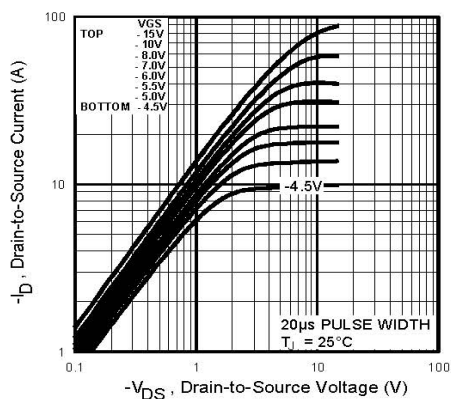
Fig 12. Typical Output Characteristics, T_J = 25^\circ C
