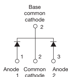
VS-MURB1020CT-1PbF
