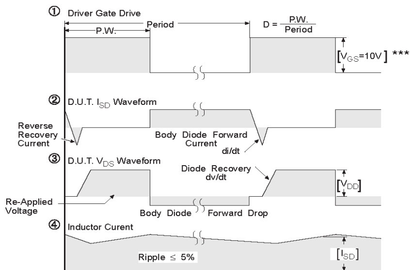
Fig 14. For P-Channel HEXFETS
