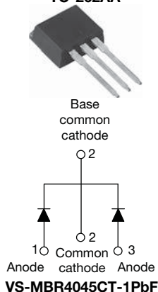
TO-262AA
