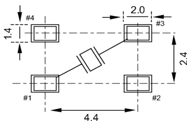
Figure 2) Land Pattern
