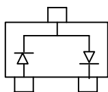
BAS40WT-04 Marking:44/K44/S42
