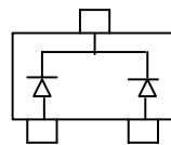
BAS40WT-05 Marking:45/K45/S43
