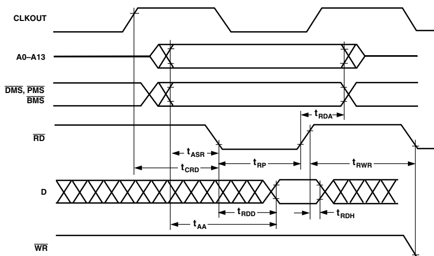
Figure 4. Memory Read
