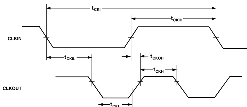
Figure 1. Clock Signals
