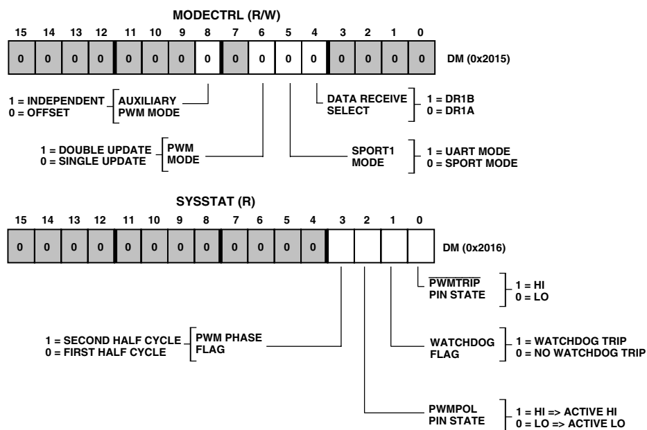
Figure 42. Structure of Registers of ADMC401
