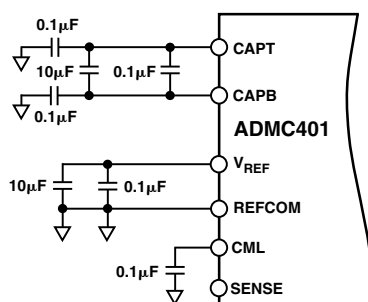
Figure 20. Recommended Capacitor Decoupling Networks for the ADCMC401
