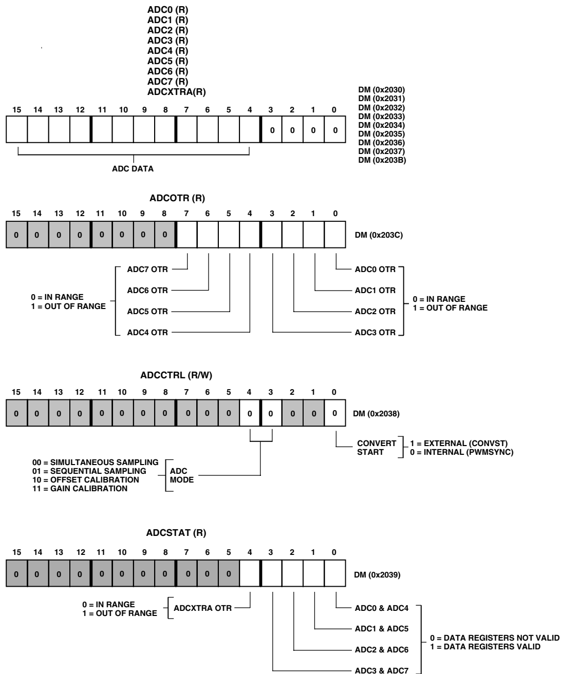
Figure 35. Structure of Registers of the ADMC401
