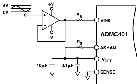
Figure 18. Typical Single-Ended Input Configuration for ADC401
