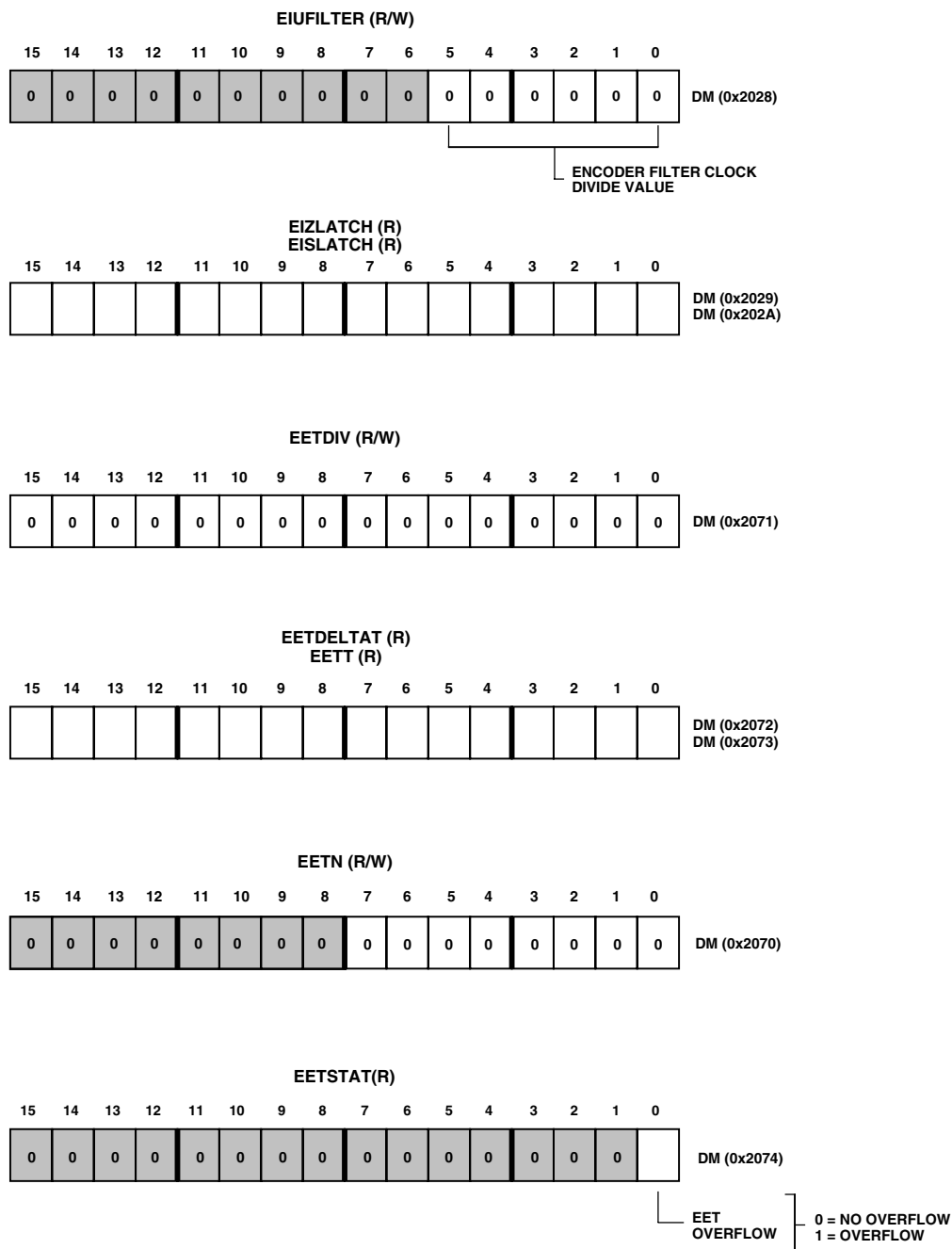
Figure 38. Structure of Registers of ADMC401
