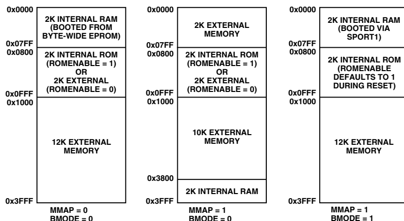
Figure 11. Program Memory Map of ADMC401
