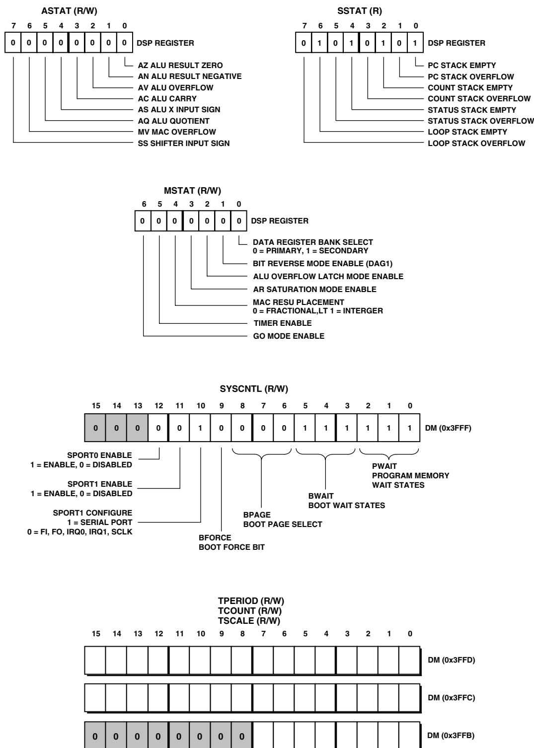
Figure 44 Structure of Registers of ADMC401
