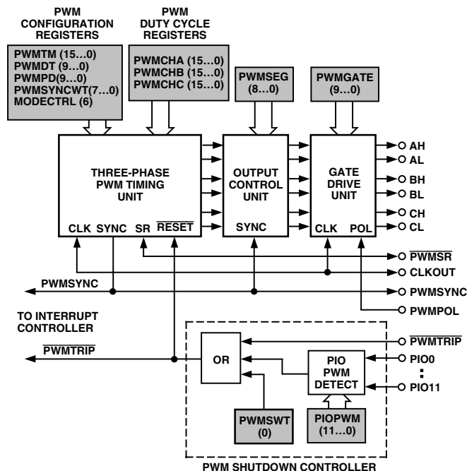
Figure 21. Overview of the ADCM401 PWM Controller
