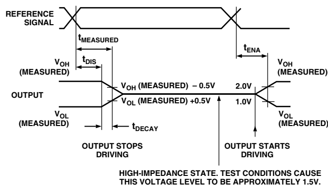
Figure 8. Output Enable/Disable
