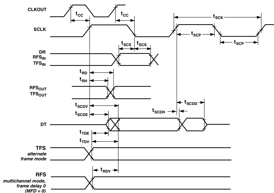
Figure 6. Serial Ports
