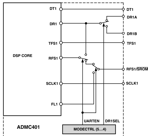
Figure 34. Internal Multiplexing of SPORT1 Pins
