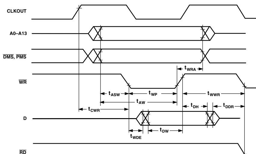
Figure 5. Memory Write
