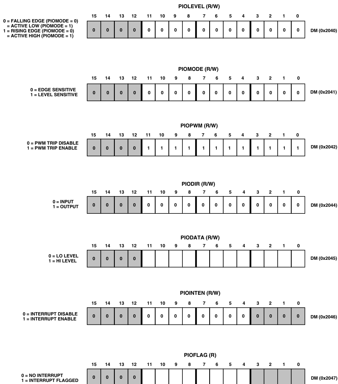
Figure 39. Structure of Registers of ADMC401
