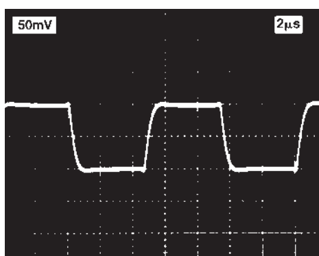
Figure 3b. Inverting Step Response
