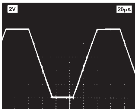
Figure 3a. Inverting Step Response
