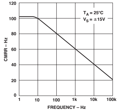
TPC 9. CMRR vs. Frequency
