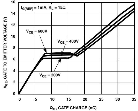
Figure 14. Gate Charge
