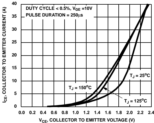
Figure 5. Collector to Emitter On-State Voltage
