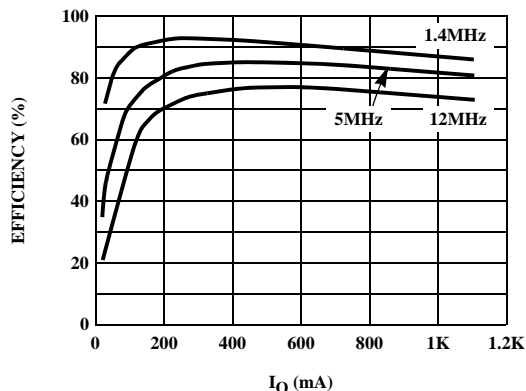
FIGURE 19. EFFICIENCY vs I_O (PWM MODE)
