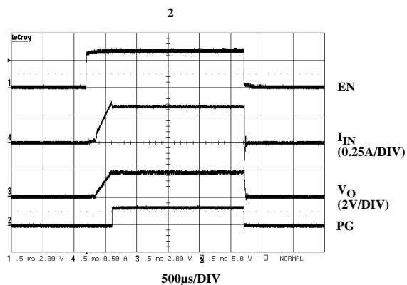
FIGURE 11. ENABLE AND SHUT-DOWN
