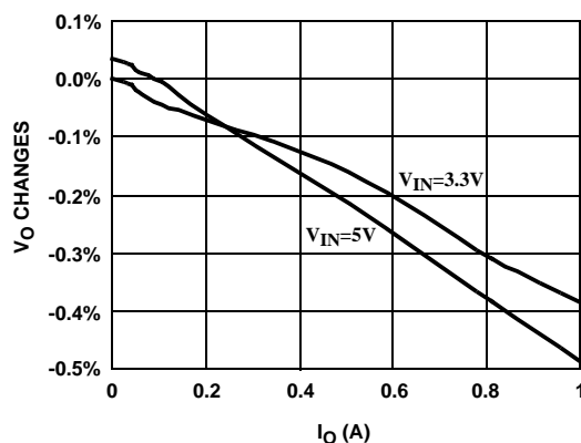
FIGURE 6. LOAD REGULATIONS (PWM MODE)
