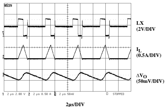
FIGURE 12. PFM STEADY-STATE OPERATION WAVEFORM ( I_O = 100mA )
