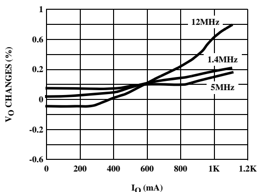
FIGURE 20. LOAD REGULATION (PWM MODE)
