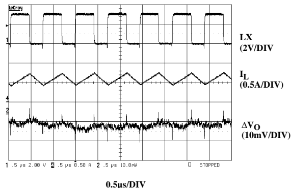
FIGURE 13. PWM STEADY-STATE OPERATION ( I_O = 600mA )
