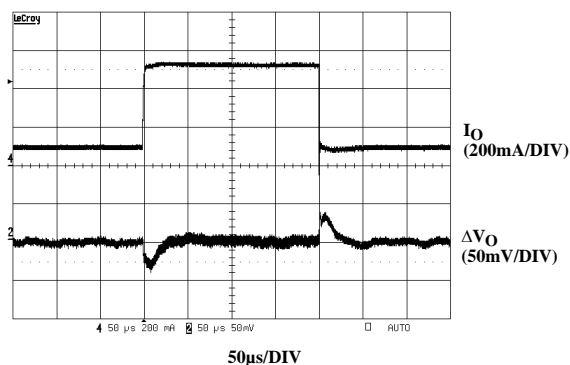
FIGURE 18. PWM LOAD TRANSIENT RESPONSE (100mA TO 500mA)
