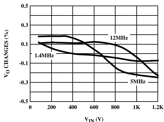
FIGURE 21. LINE REGULATION @ 500mA (PWM MODE)
