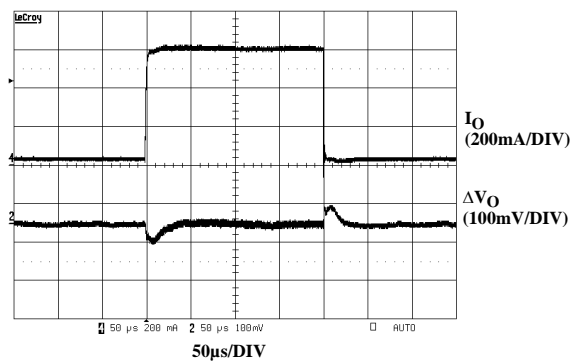
FIGURE 17. PWM LOAD TRANSIENT RESPONSE (30mA TO 600mA)
