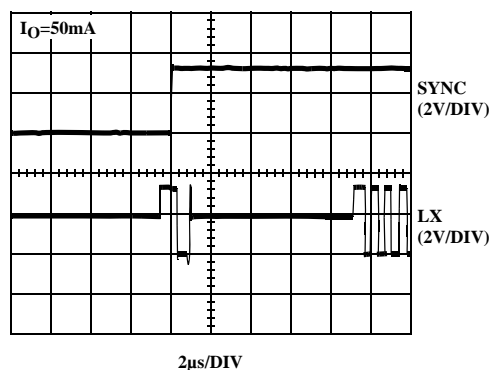
FIGURE 23. PFM-PWM TRANSITION TIME
