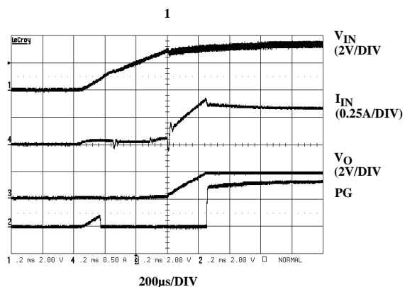
FIGURE 10. START-UP AT I_O = 600mA
