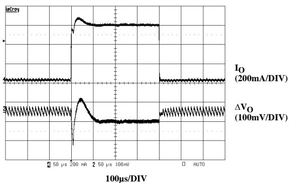
FIGURE 16. LOAD TRANSIENT RESPONSE (22mA TO 600mA)
