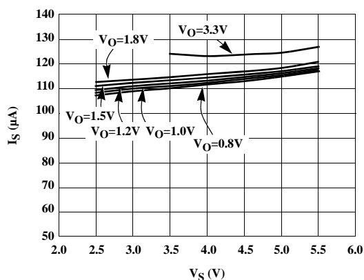
FIGURE 9. NO LOAD QUIESCENT CURRENT (PFM MODE)
