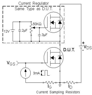
Fig 9b. Gate Charge Test Circuit
