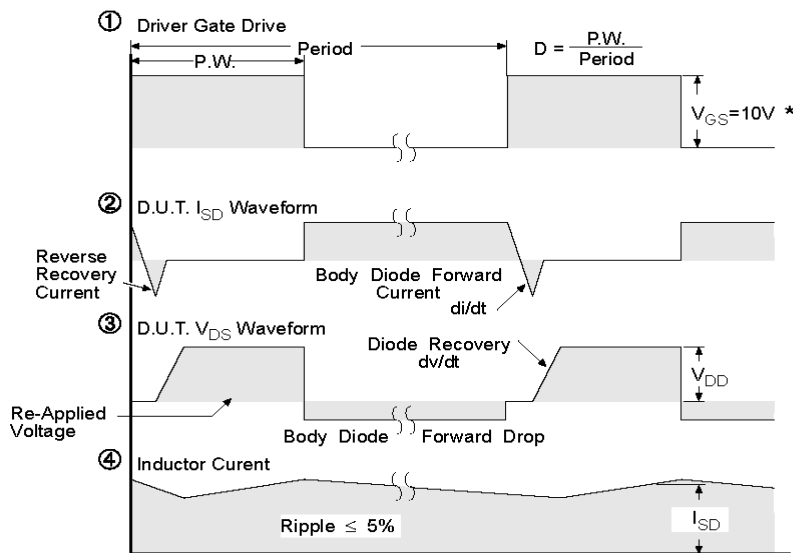
Fig 12. For N-Channel HEXFETS
