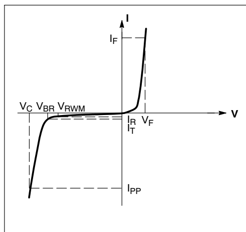
Uni-Directional TVS
