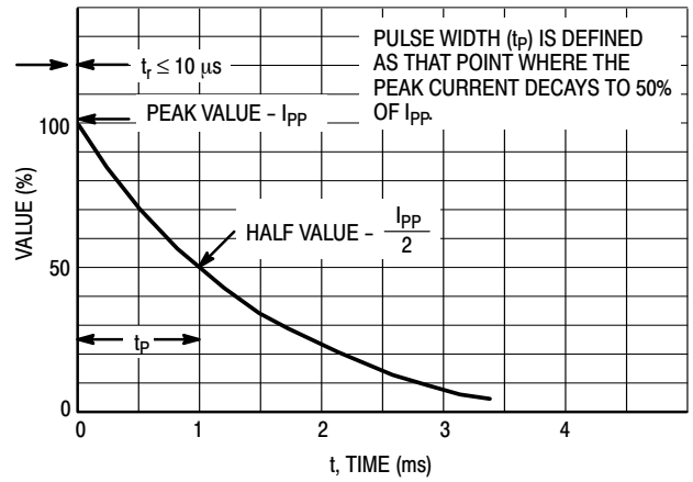
Figure 4. Pulse Waveform
