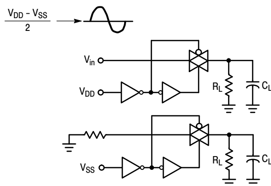
Figure 4. Channel Separation
