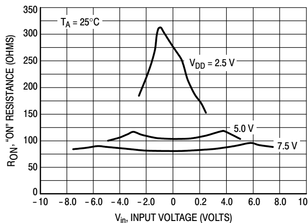
Figure 11. Comparison at 25^\circ\text{C} , V_{DD} = -V_{SS}
