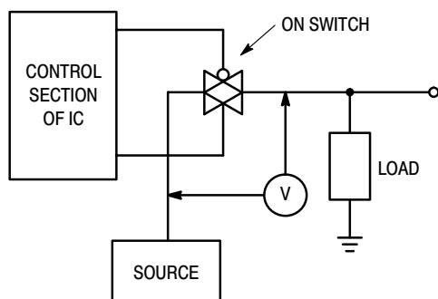
Figure 1. \Delta V Across Switch
