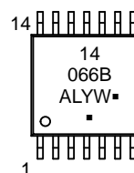
TSSOP-14
