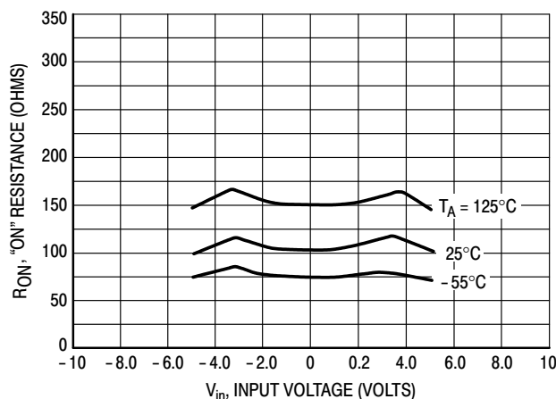
Figure 9. V_{DD} = 5.0 \text{ V} , V_{SS} = -5.0 \text{ V}
