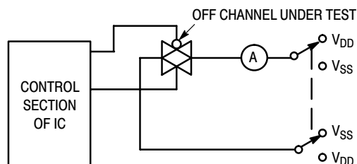
Figure 6. Off Channel Leakage
