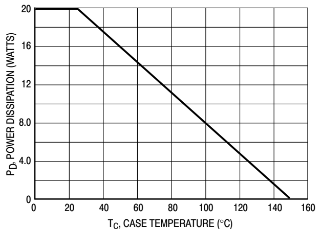
Figure 5. Power Derating
