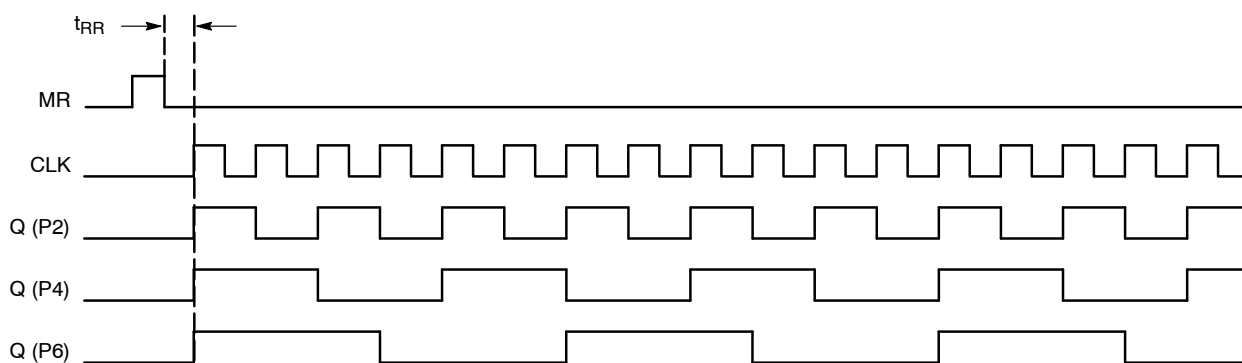
Figure 3. Timing Diagram
