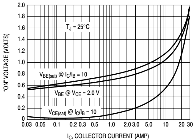
Figure 3. "On" Voltages
