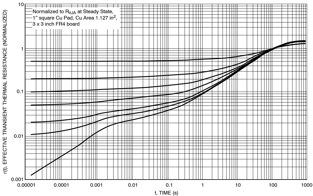
Figure 14. Thermal Response
