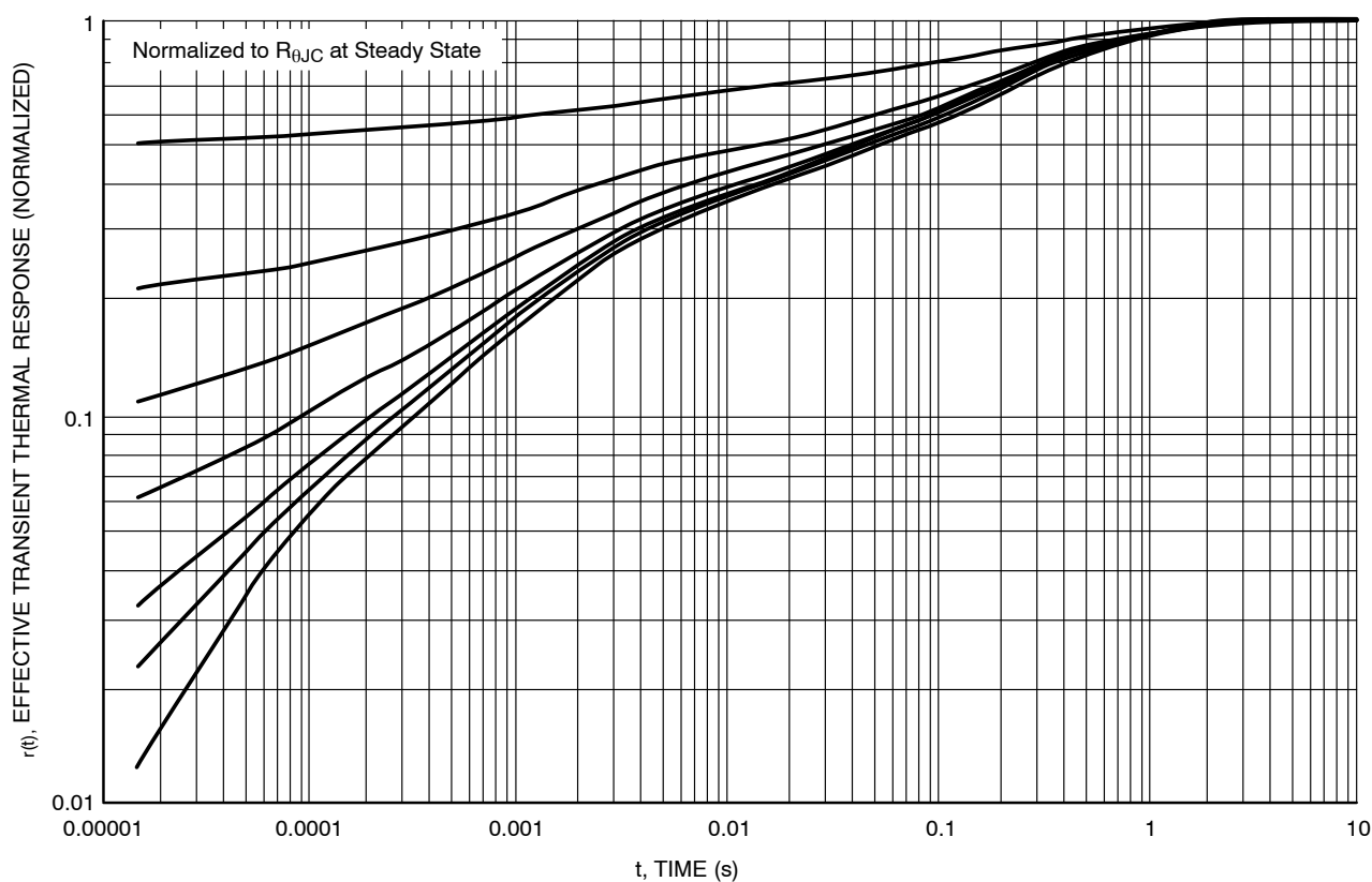
Figure 13. Thermal Response
