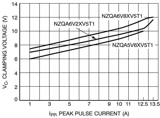
Figure 3. Clamping Voltage versus Peak Pulse Current
