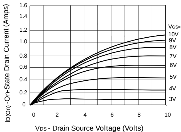
Saturation Characteristics
