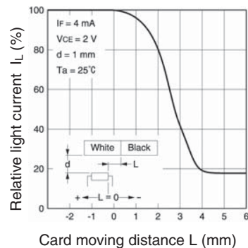
Relative Collector Current vs. Card Moving Distance (2)
