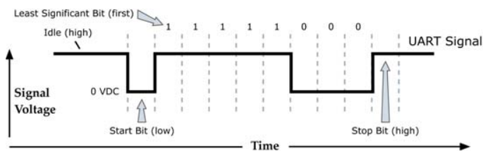
Figure 2-02. UART data packet 0x1F (decimal number "31") as transmitted through the RF module
