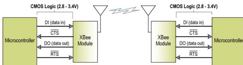
Figure 2-01. System Data Flow Diagram in a UART-interfaced environment
