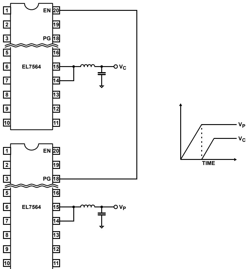
FIGURE 26. OFFSET TRACKING
