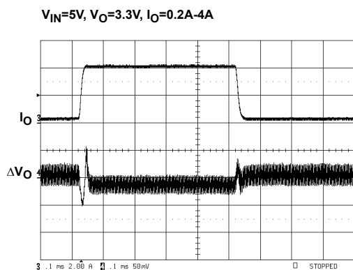
FIGURE 15. TRANSIENT RESPONSE
