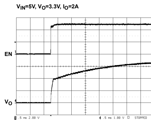
FIGURE 18. RELEASING EN
