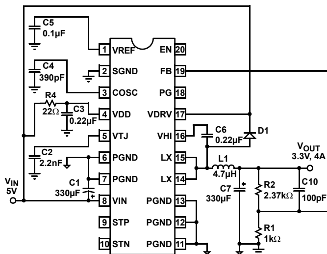
EL7564 [20-PIN SO (0.300")] TOP VIEW
