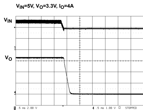
FIGURE 17. POWER-DOWN
