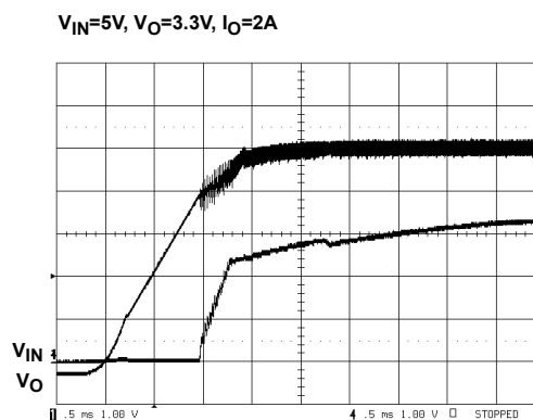
FIGURE 16. POWER-UP
