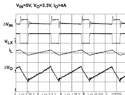
FIGURE 14. SWITCHING WAVEFORMS
