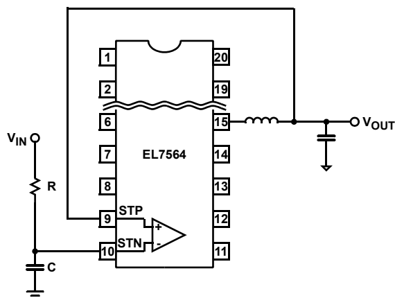
FIGURE 27. EXTERNAL SOFT START
