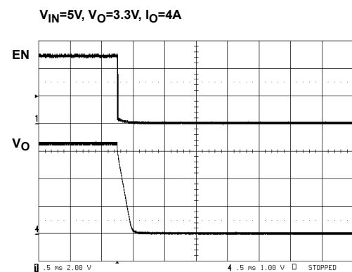
FIGURE 19. SHUT-DOWN
