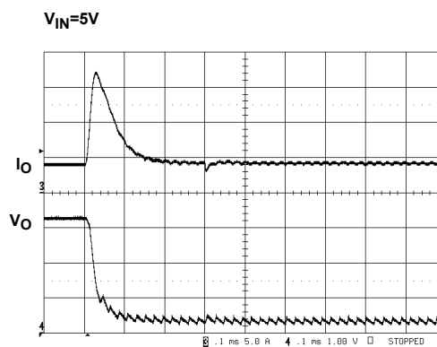
FIGURE 20. SHORT-CIRCUIT PROTECTION
