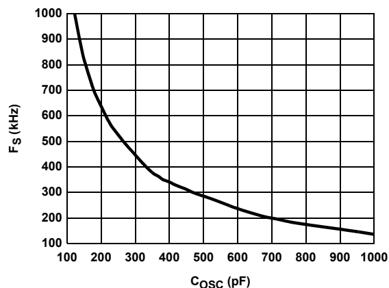
FIGURE 10. SWITCHING FREQUENCY vs C_{OSC}
