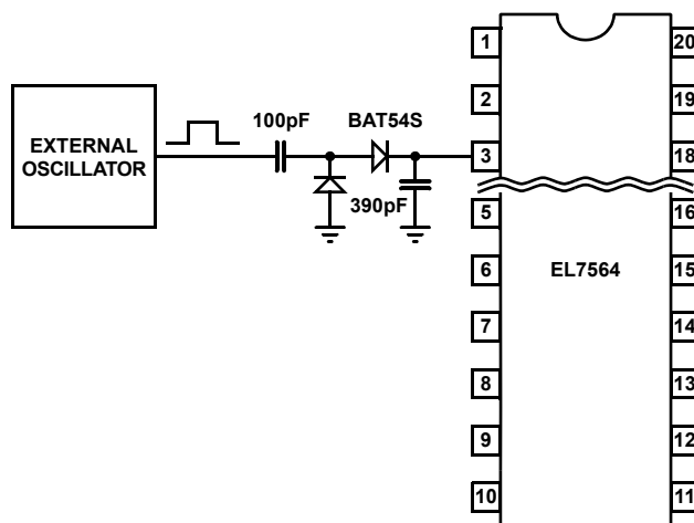
FIGURE 23. OSCILLATOR SYNCHRONIZATION
