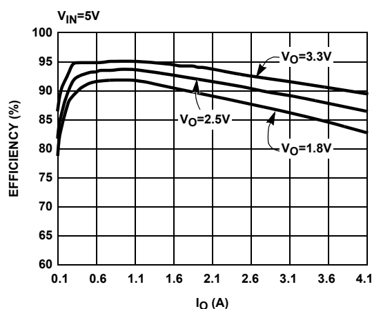
FIGURE 2. EL7564CRE EFFICIENCY
