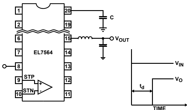
FIGURE 28. START-UP DELAY
