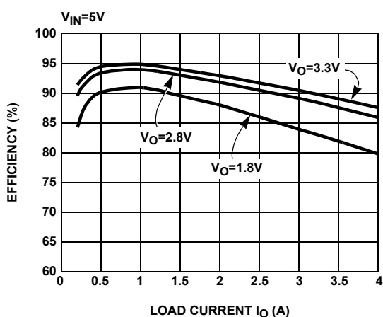
FIGURE 1. EL7564CM EFFICIENCY
