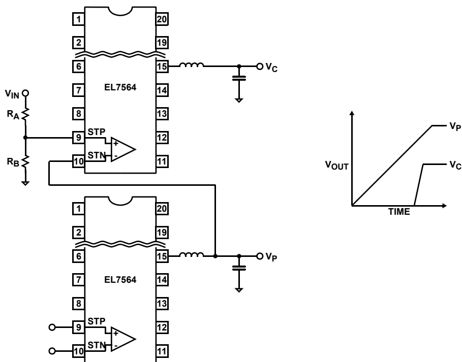
FIGURE 25. OFFSET POWER TRACKING
