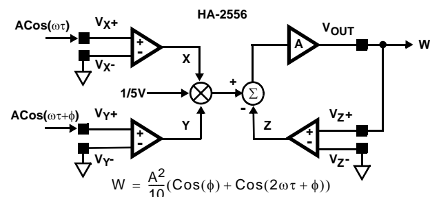
FIGURE 8. PHASE DETECTION
