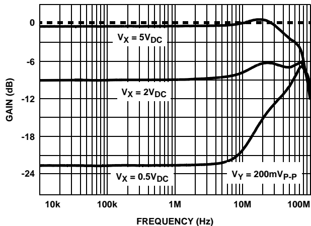
FIGURE 34. Y-CHANNEL BANDWIDTH vs X-CHANNEL
