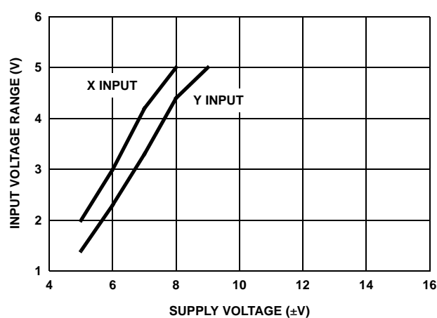
FIGURE 43. INPUT VOLTAGE RANGE vs SUPPLY VOLTAGE
