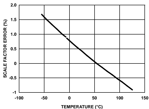
FIGURE 42. SCALE FACTOR ERROR vs TEMPERATURE
