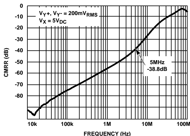
FIGURE 36. Y-CHANNEL CMRR vs FREQUENCY
