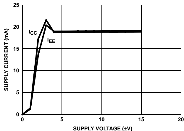
FIGURE 45. SUPPLY CURRENT vs SUPPLY VOLTAGE
