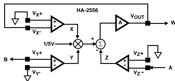
FIGURE 3. DIVIDER
