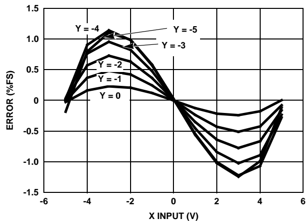
FIGURE 25. X-CHANNEL MULTIPLIER ERROR
