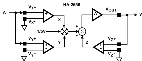
FIGURE 4. SQUARE
