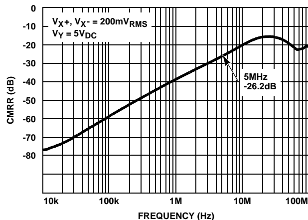
FIGURE 37. X-CHANNEL CMRR vs FREQUENCY
