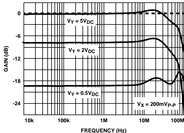
FIGURE 35. X-CHANNEL BANDWIDTH vs Y-CHANNEL
