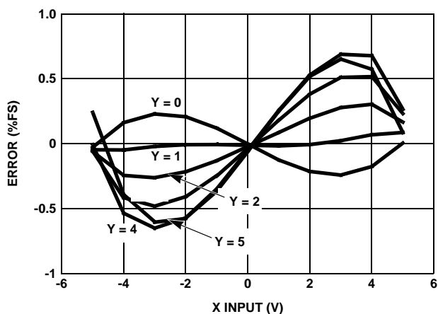
FIGURE 24. X-CHANNEL MULTIPLIER ERROR
