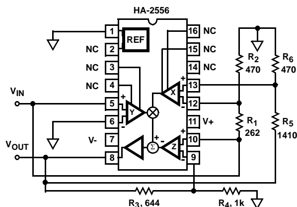
FIGURE 22. SINE-FUNCTION GENERATOR
