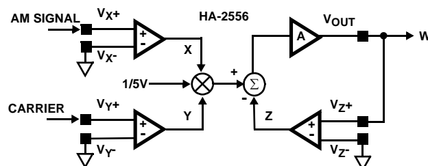
FIGURE 7. SYNCHRONOUS AM DETECTION
