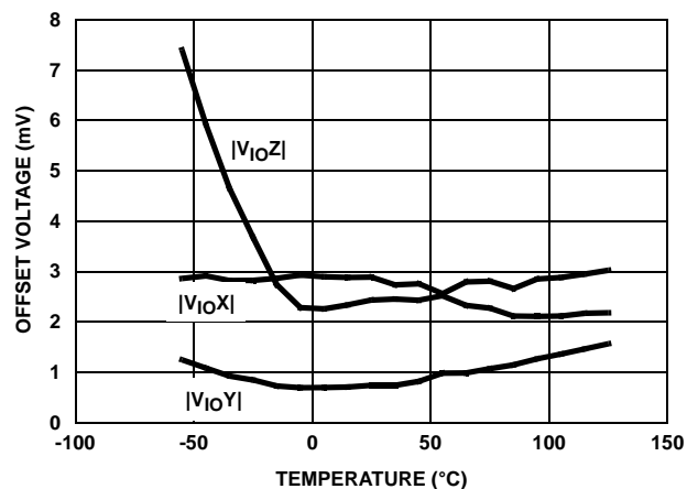
FIGURE 40. OFFSET VOLTAGE vs TEMPERATURE
