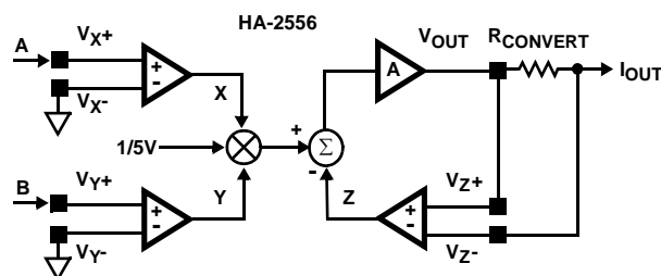
FIGURE 10. CURRENT OUTPUT
