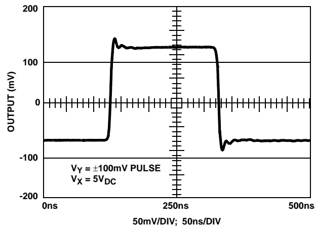
FIGURE 29. SMALL SIGNAL RESPONSE
