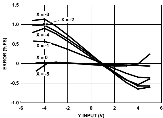
FIGURE 26. Y-CHANNEL MULTIPLIER ERROR
