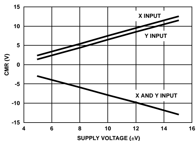
FIGURE 44. INPUT COMMON MODE RANGE vs SUPPLY VOLTAGE
