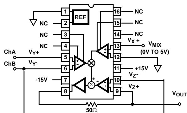
FIGURE 11. VIDEO FADER
