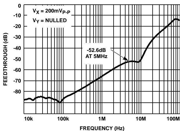
FIGURE 38. FEEDTHROUGH vs FREQUENCY
