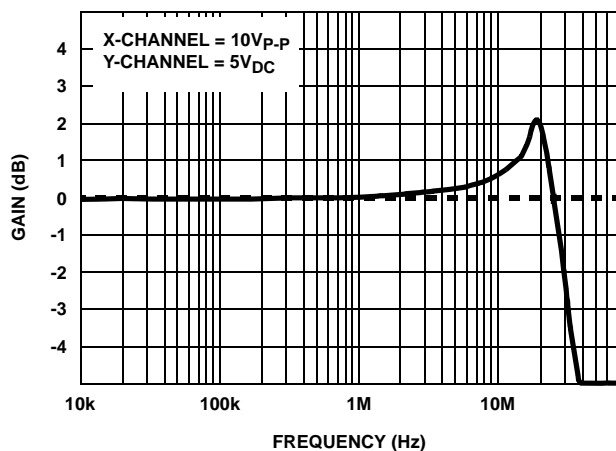
FIGURE 32. X-CHANNEL FULL POWER BANDWIDTH
