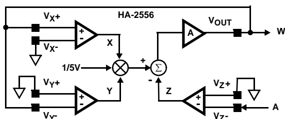
FIGURE 5. SQUARE ROOT (FOR A > 0 )
