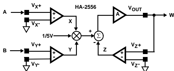
FIGURE 2. MULTIPLIER
