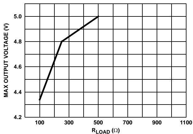
FIGURE 46. OUTPUT VOLTAGE vs R_{LOAD}
