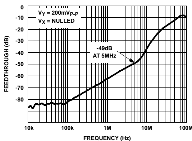
FIGURE 39. FEEDTHROUGH vs FREQUENCY
