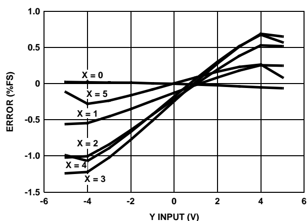
FIGURE 27. Y-CHANNEL MULTIPLIER ERROR
