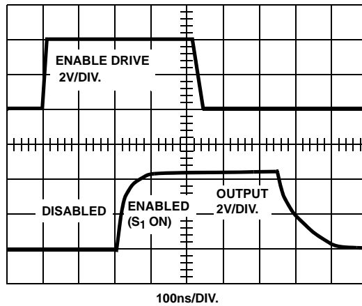
FIGURE 8C. WAVEFORMS
