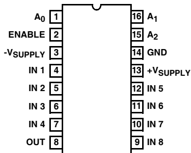
HI-508A (CERDIP, PDIP) TOP VIEW
