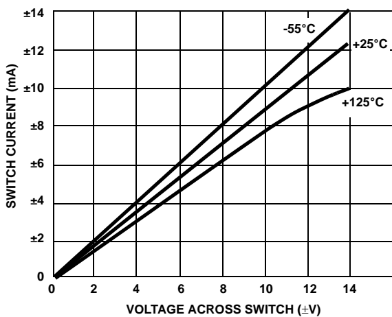
FIGURE 4A. ON CHANNEL CURRENT vs VOLTAGE
