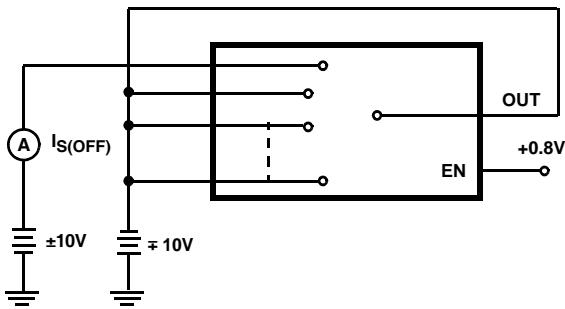
FIGURE 2C. I_{S(\text{OFF})} TEST CIRCUIT (NOTE 13)
