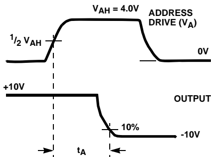
FIGURE 6C. MEASUREMENT POINTS
