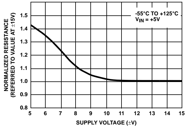
FIGURE 1C. NORMALIZED ON RESISTANCE vs SUPPLY VOLTAGE
