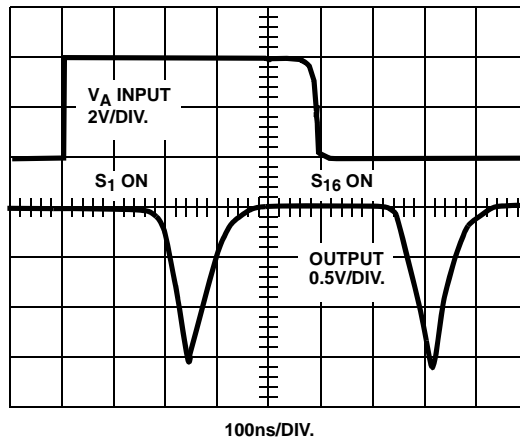
FIGURE 7C. WAVEFORMS
