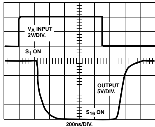
FIGURE 6D. WAVEFORMS
