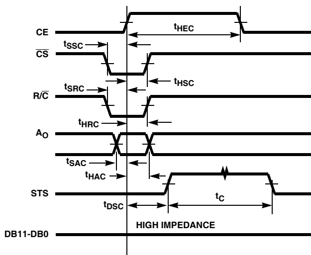
FIGURE 3. CONVERT START TIMING
