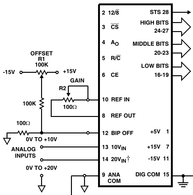
FIGURE 1. UNIPOLAR CONNECTIONS
