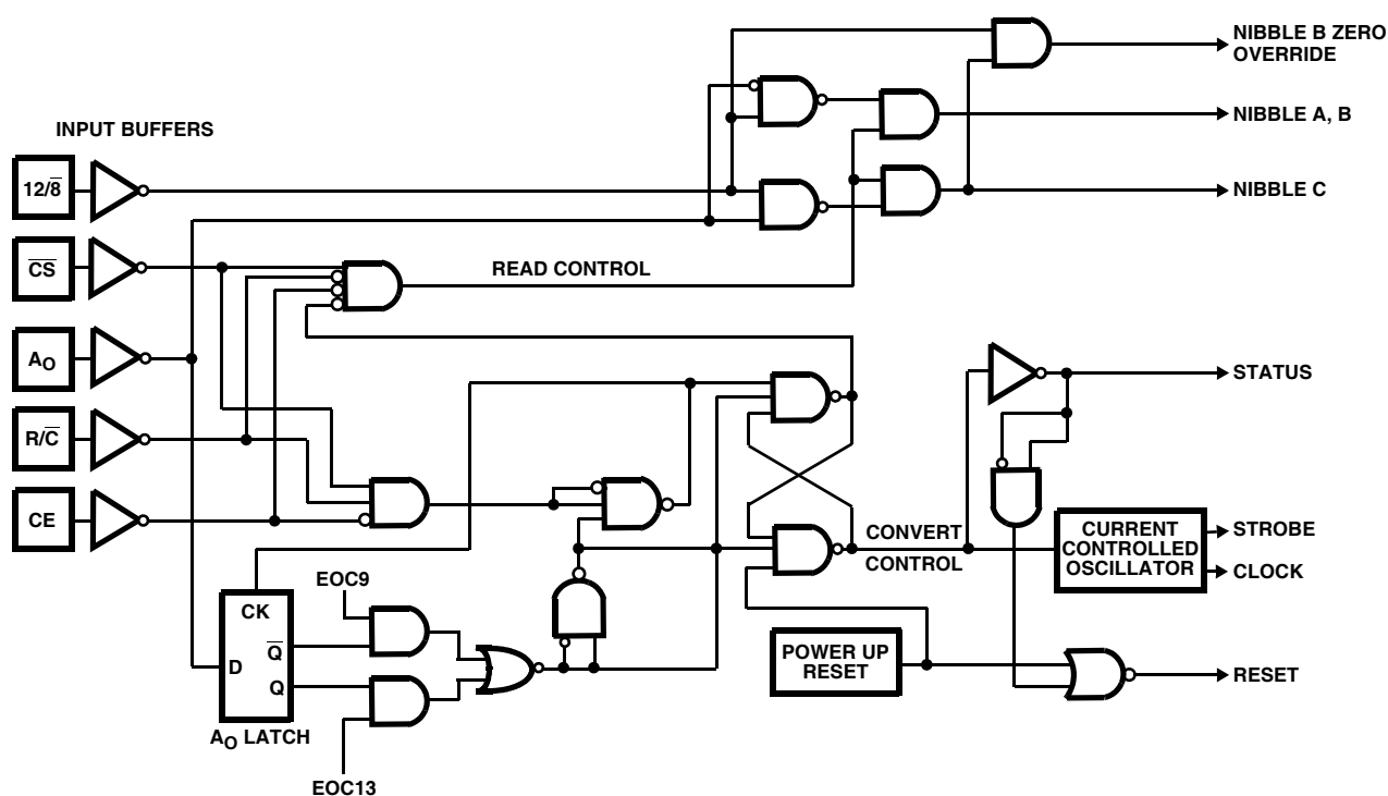
FIGURE 6. HI-X74A CONTROL LOGIC
