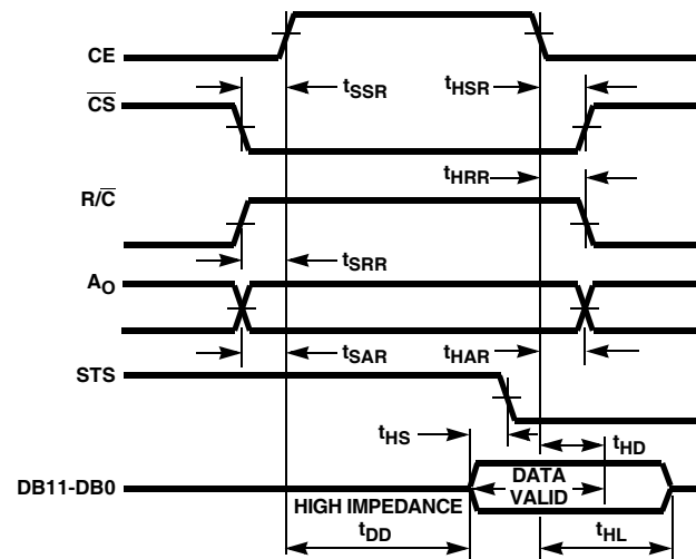
FIGURE 4. READ CYCLE TIMING
