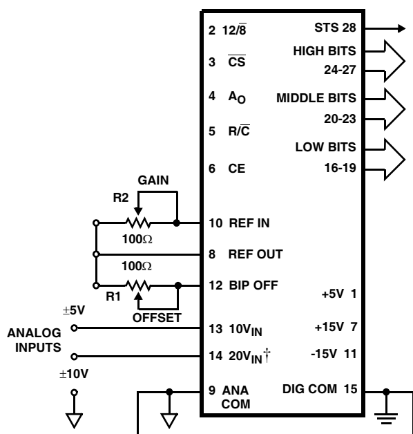
FIGURE 2. BIPOLAR CONNECTIONS
