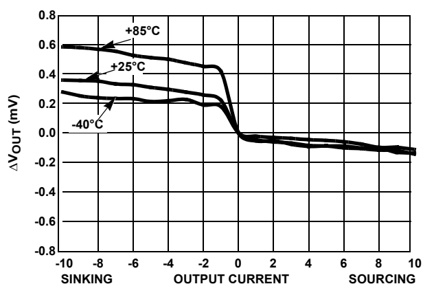
FIGURE 50. LOAD REGULATION OVER-TEMPERATURE
