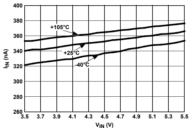
FIGURE 100. I_{IN} vs V_{IN} OVER-TEMPERATURE
