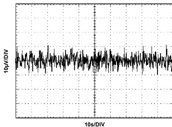
FIGURE 42. V_{OUT} NOISE
