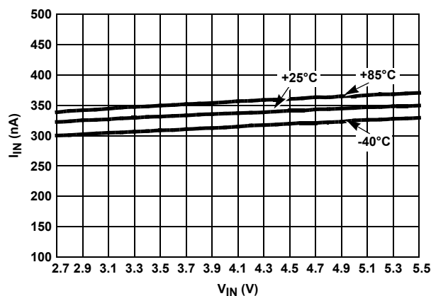
FIGURE 58. I_{IN} vs V_{IN} OVER-TEMPERATURE
