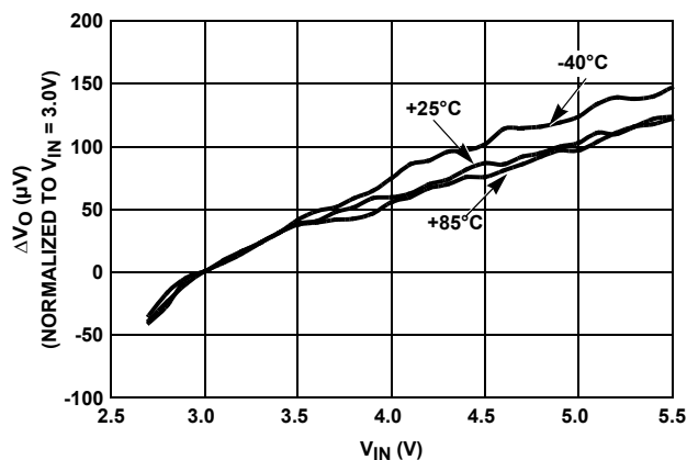
FIGURE 74. LINE REGULATION OVER-TEMPERATURE
