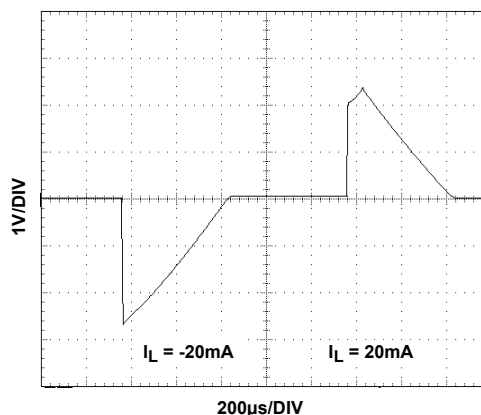
FIGURE 96. LOAD TRANSIENT RESPONSE
