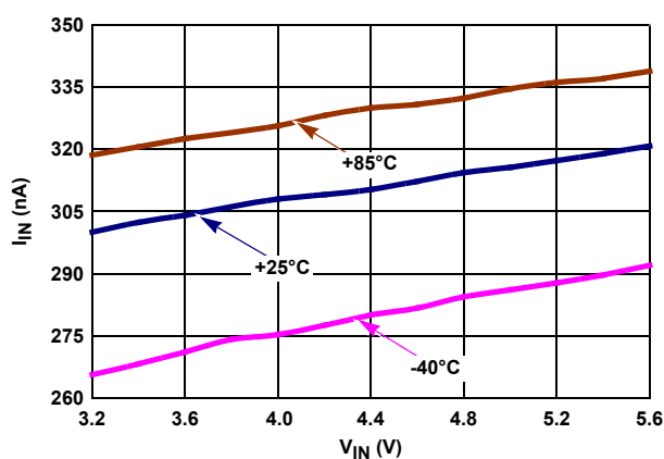
FIGURE 85. I_{IN} vs V_{IN} OVER-TEMPERATURE
