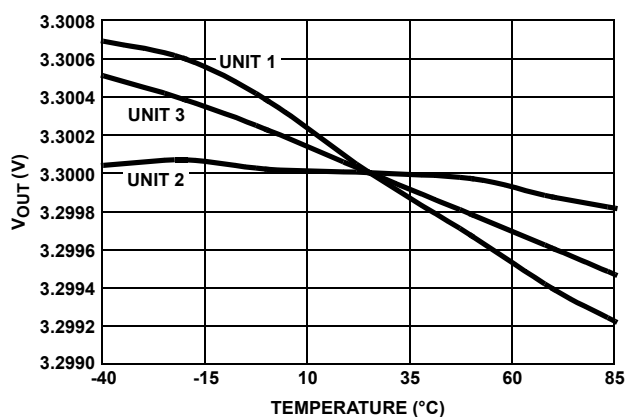
FIGURE 101. V_{OUT} vs TEMPERATURE NORMALIZED TO +25^\circ C
