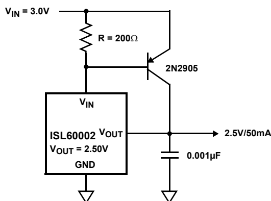
FIGURE 121. PRECISION 2.5V 50mA REFERENCE
