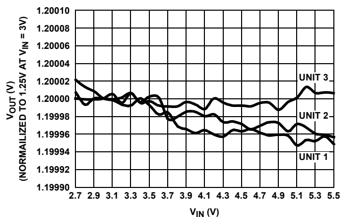
FIGURE 18. LINE REGULATION, 3 UNITS
