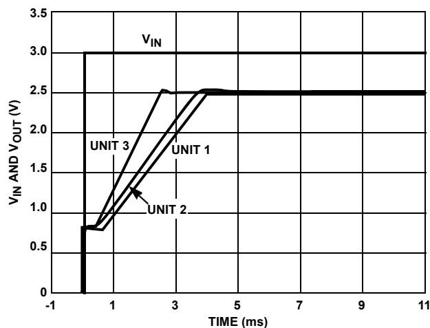
FIGURE 120. TURN-ON TIME
