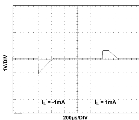
FIGURE 94. LOAD TRANSIENT RESPONSE
