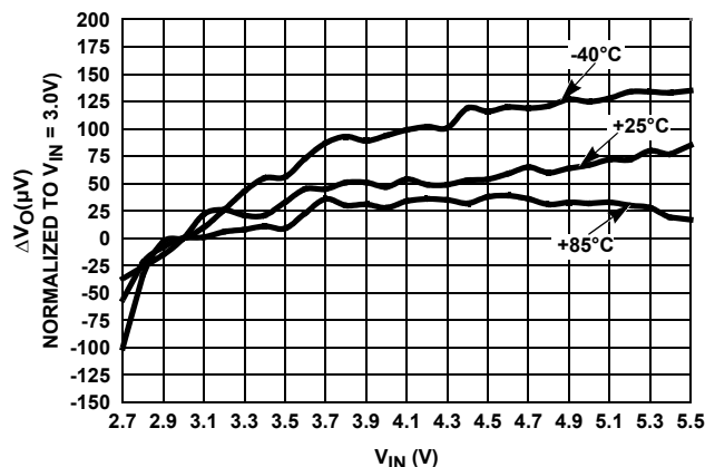
FIGURE 60. LINE REGULATION OVER-TEMPERATURE
