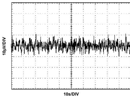
FIGURE 83. V_{OUT} NOISE
