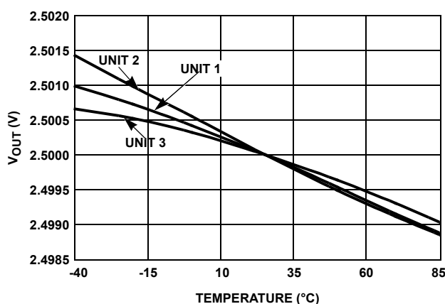
FIGURE 72. V_{OUT} vs TEMPERATURE NORMALIZED TO +25^\circ C
