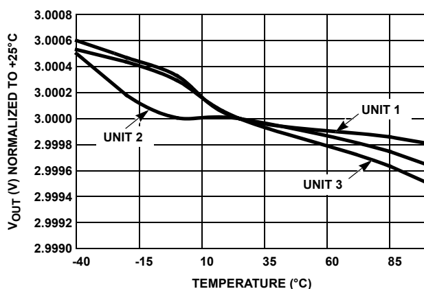
FIGURE 86. V_{OUT} vs TEMPERATURE NORMALIZED TO +25^\circ C
