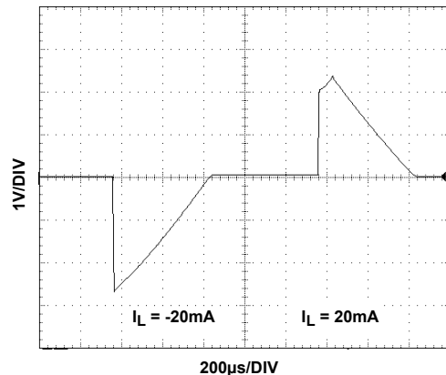
FIGURE 112. LOAD TRANSIENT RESPONSE
