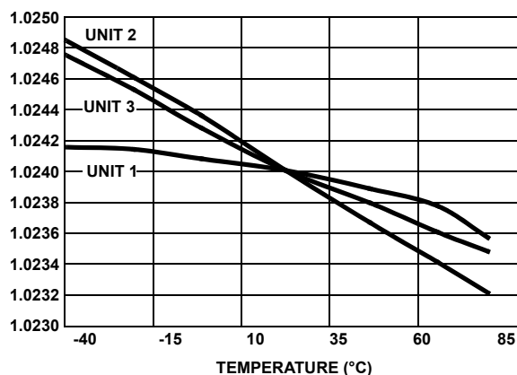
FIGURE 6. V_{OUT} vs TEMPERATURE NORMALIZED to +25^\circ C
