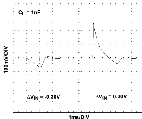
FIGURE 90. LINE TRANSIENT RESPONSE
