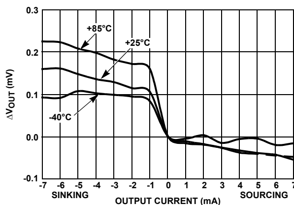
FIGURE 37. LOAD REGULATION
