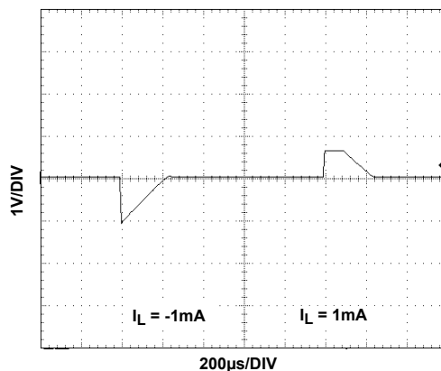
FIGURE 110. LOAD TRANSIENT RESPONSE
