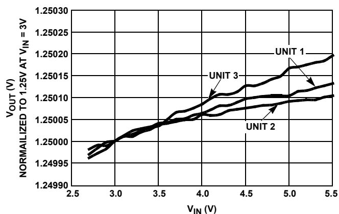
FIGURE 32. LINE REGULATION, 3 UNITS
