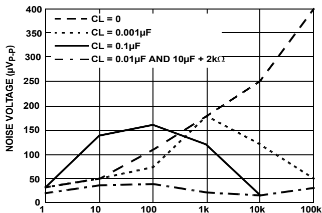
FIGURE 118. NOISE REDUCTION
