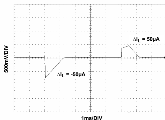
FIGURE 52. LOAD TRANSIENT RESPONSE
