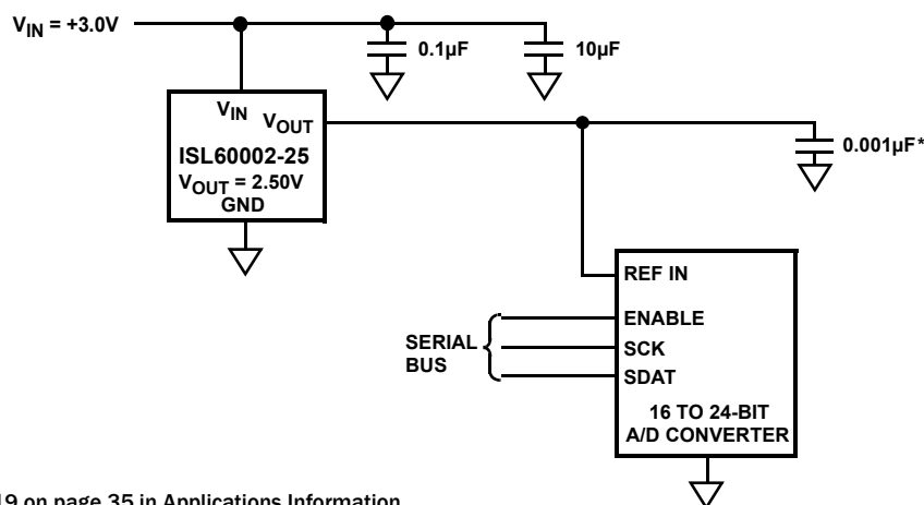
FIGURE 1. TYPICAL APPLICATION
