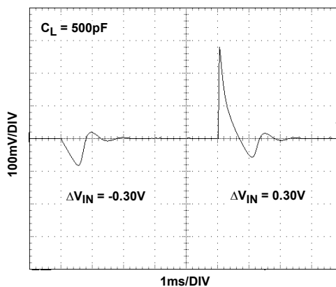
FIGURE 21. LINE TRANSIENT RESPONSE WITH CAPACITIVE LOAD
