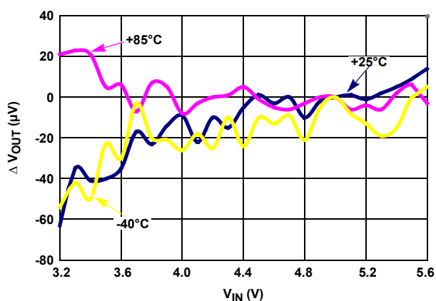
FIGURE 88. LINE REGULATION OVER-TEMPERATURE
