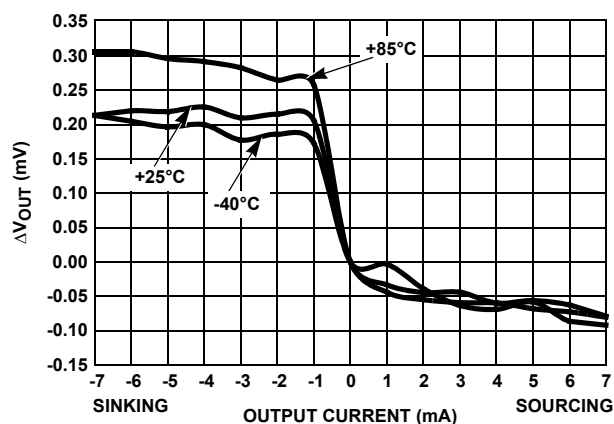
FIGURE 92. LOAD REGULATION OVER-TEMPERATURE
