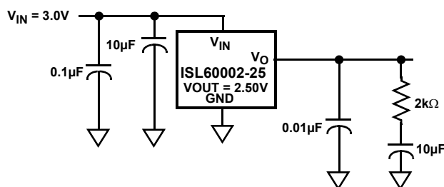
FIGURE 119. NOISE REDUCTION NETWORK
