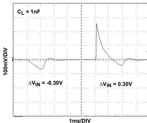
FIGURE 105. LINE TRANSIENT RESPONSE
