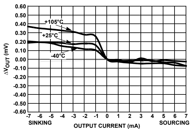
FIGURE 107. LOAD REGULATION
