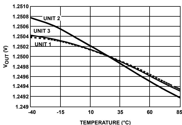
FIGURE 31. V_{OUT} vs TEMPERATURE NORMALIZED TO +25^\circ C
