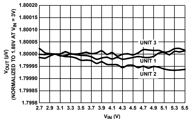
FIGURE 45. LINE REGULATION (3 REPRESENTATIVE UNITS)
