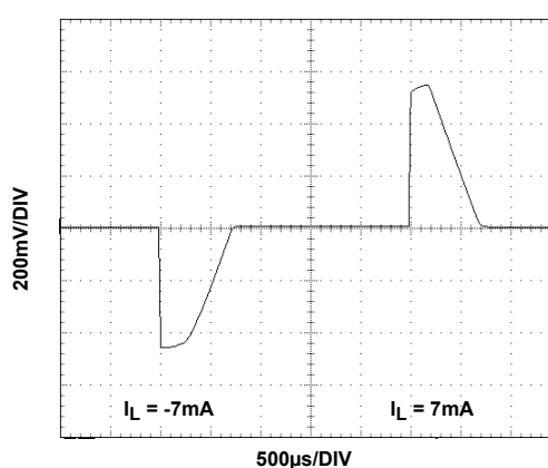
FIGURE 39. LOAD TRANSIENT RESPONSE
