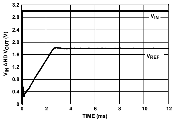
FIGURE 54. TURN-ON TIME (+25°C)
