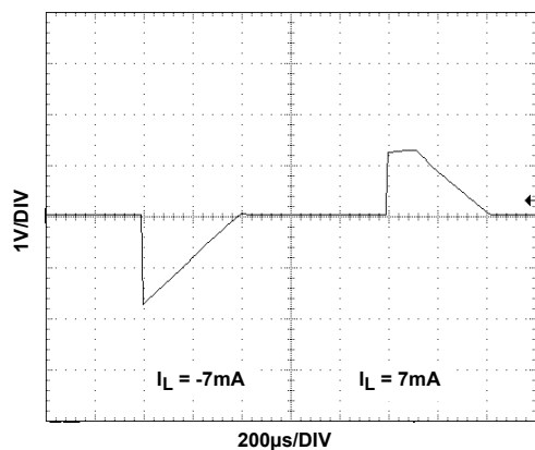
FIGURE 95. LOAD TRANSIENT RESPONSE
