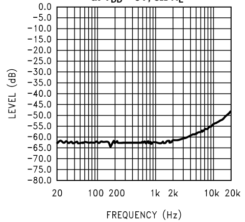
Figure 11. Input Floating
