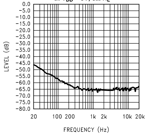
Figure 10. Input terminated with 10Ω
