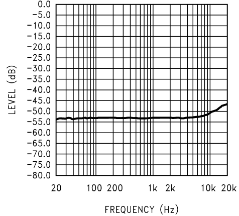
Figure 15. Input Floating
