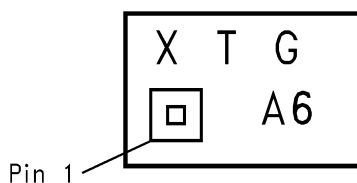
8 Bump DSBGA Marking (Top View) X - Date Code T - Dice Traceability G - Boomer Family A6 - LM4904ITL
