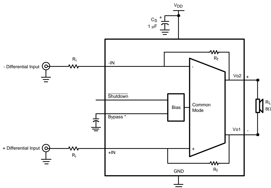
Figure 1. Typical Audio Amplifier Application Circuit
