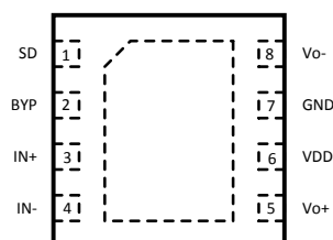
Figure 2. 8 Pin WSON Package Top View See Package Number NGQ0008A
