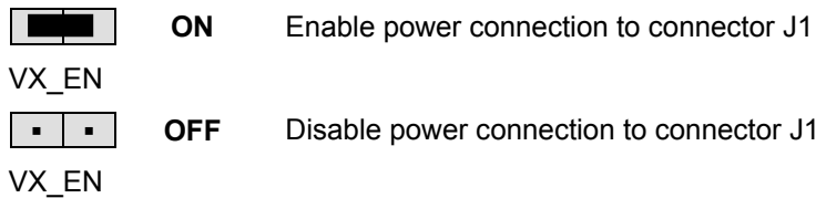
Figure 2. VX_EN Option Header
