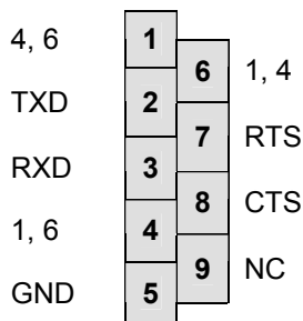
Figure 4: COM Connector
