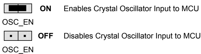
Figure 3: OSC_EN Option Header
