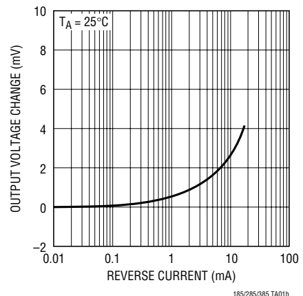
Reverse Voltage Change with Current
