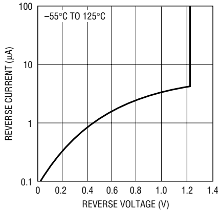
Reverse Characteristics
