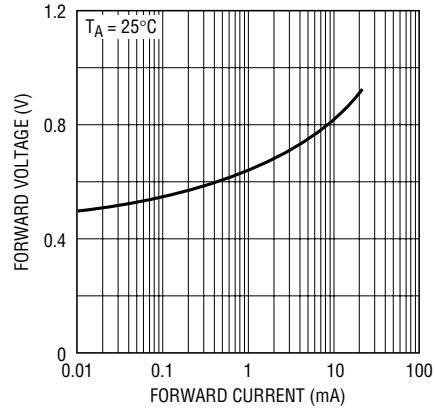
Forward Characteristics
