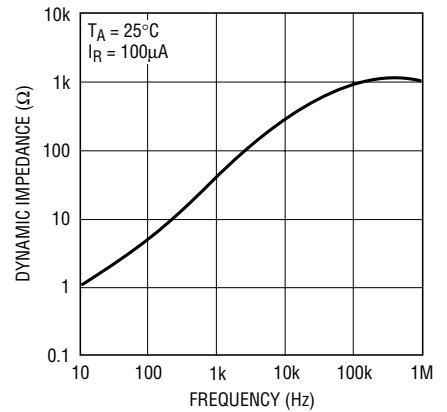
Reverse Dynamic Impedance
