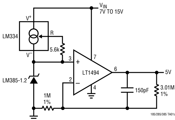
Micropower 5V Reference
