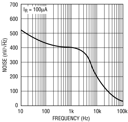
Noise Voltage
