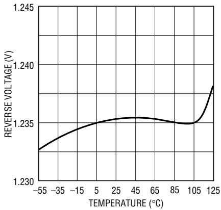
Temperature Drift
