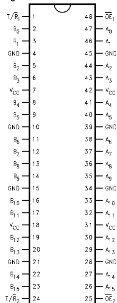
Pin Assignments for SSOP and TSSOP
