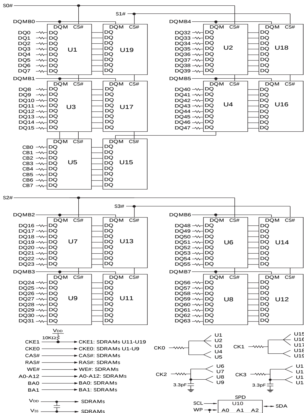
Figure 4: Functional Block Diagram – Dual Rank
