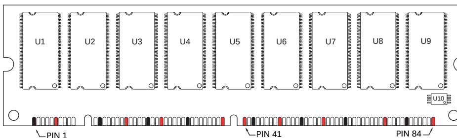
Figure 2: Pin Locations (168-Pin DIMM)
