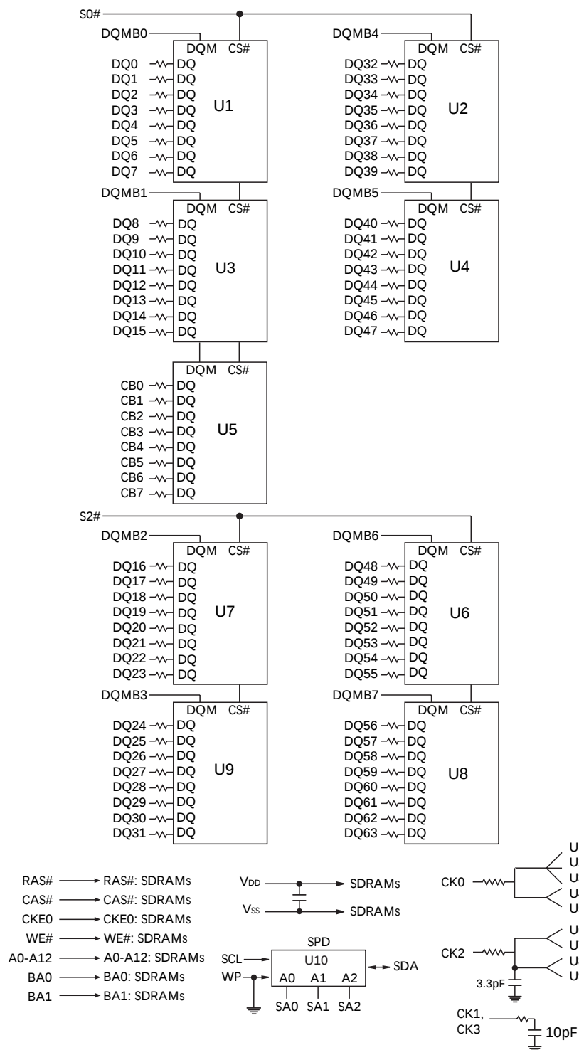
Figure 3: Functional Block Diagram – Single Rank
