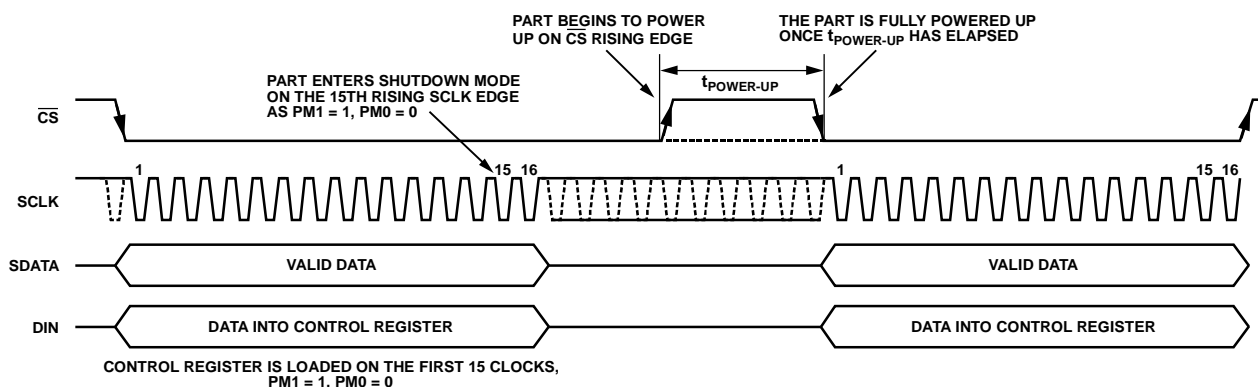
Figure 48. Entering Autoshutdown/Autostandby Mode
