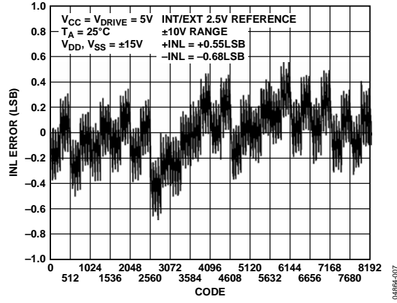
Figure 7. Typical INL True Differential Mode
