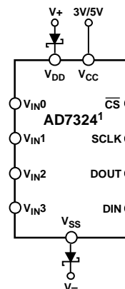
1 ADDITIONAL PINS OMITTED FOR CLARITY. 048864-05E
