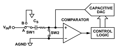
Figure 23. ADC Acquisition Phase (Single-Ended)
