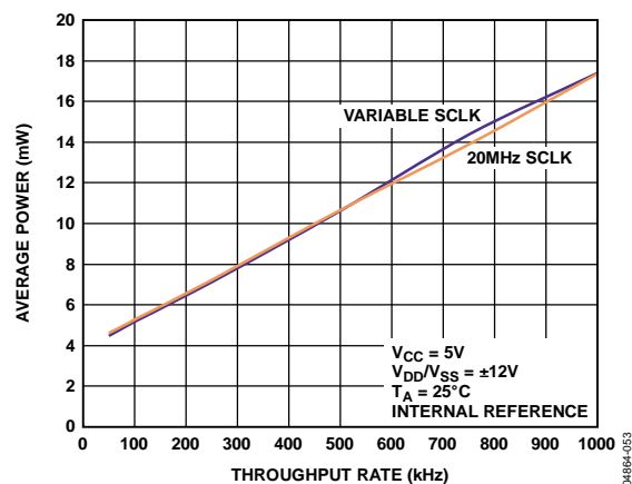
Figure 50. Power vs. Throughput Rate with 5 V V_{CC}
