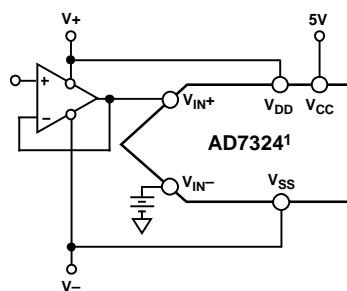
1 ADDITIONAL PINS OMITTED FOR CLARITY.
