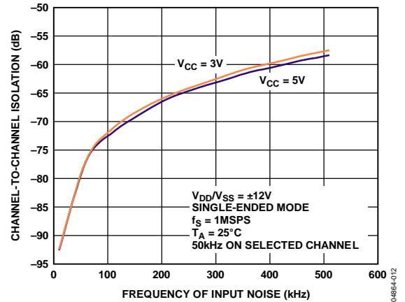
Figure 14. Channel-to-Channel Isolation
