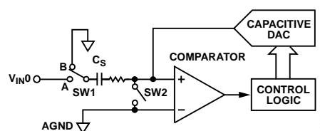
Figure 24. ADC Conversion Phase (Single-Ended)
