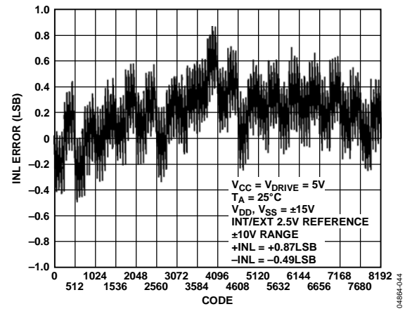
Figure 9. Typical INL Single-Ended Mode
