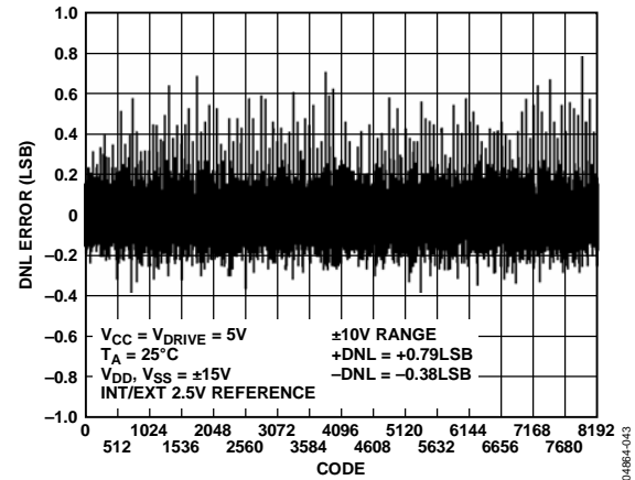
Figure 8. Typical DNL Single-Ended Mode
