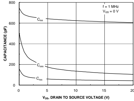
Figure 8. Capacitance Characteristics.
