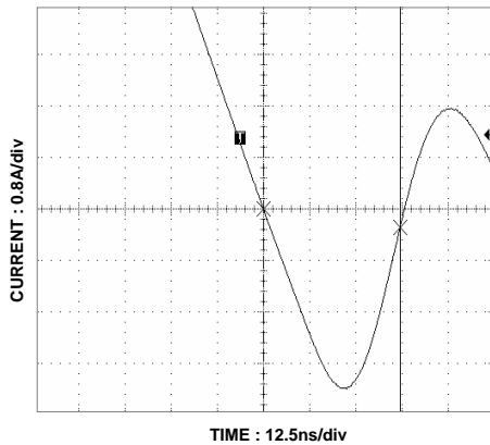
Figure 13. Non-SyncFET (FDS6688) body diode reverse recovery characteristic.
