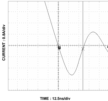
Figure 12. FDS6689S SyncFET body diode reverse recovery characteristic.
