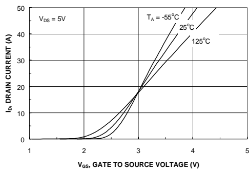
Figure 5. Transfer Characteristics.
