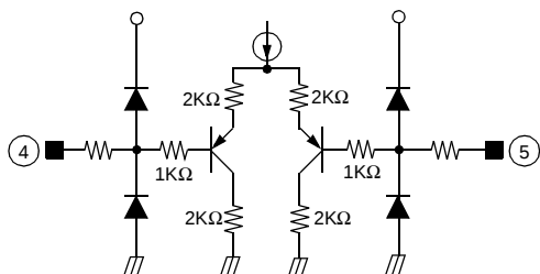
Figure 1. Error Amp Input
