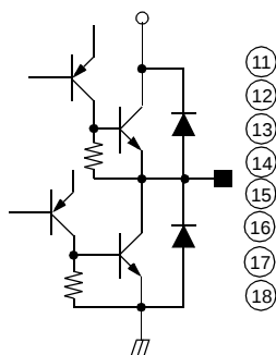
Figure 3. Power Amp Output
