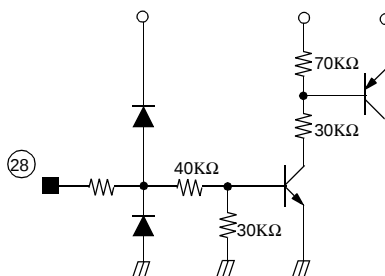
Figure 4. Stand-By Input
