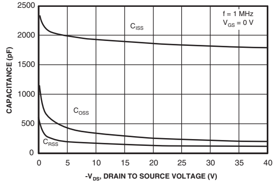
Figure 8. Capacitance Characteristics.
