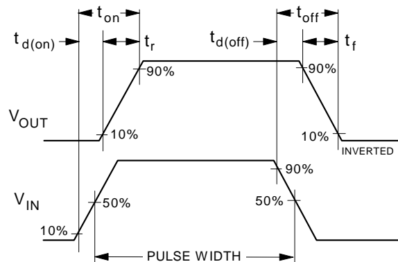
Figure 11. Switching Waveforms.
