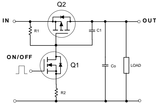
APPLICATION CIRCUIT
