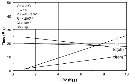
Figure 8. Switching Variation with R2 at Vin = 2.5V and R1 = 20KOhm.
