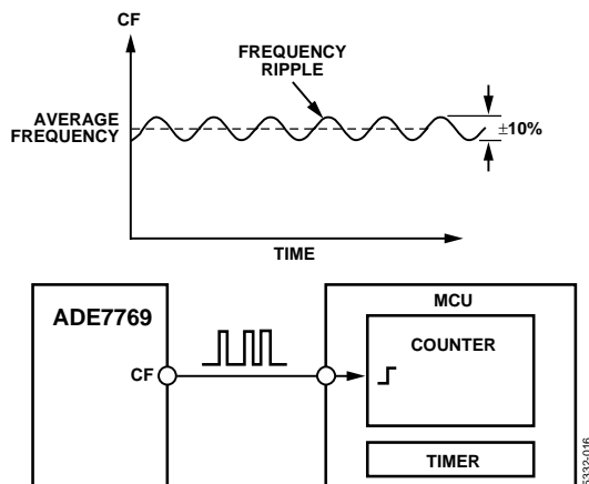
Figure 26. Interfacing the ADE7769 to an MCU
