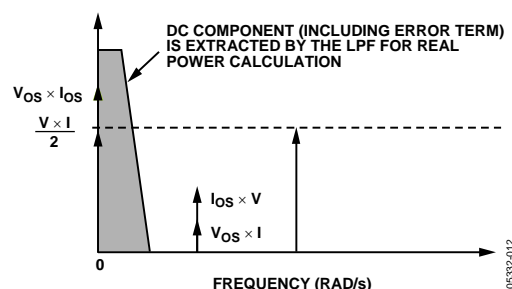
Figure 22. Effect of Channel Offset on the Real Power Calculation
