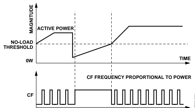
Figure 28. No-Load Indication Using ADE7769
