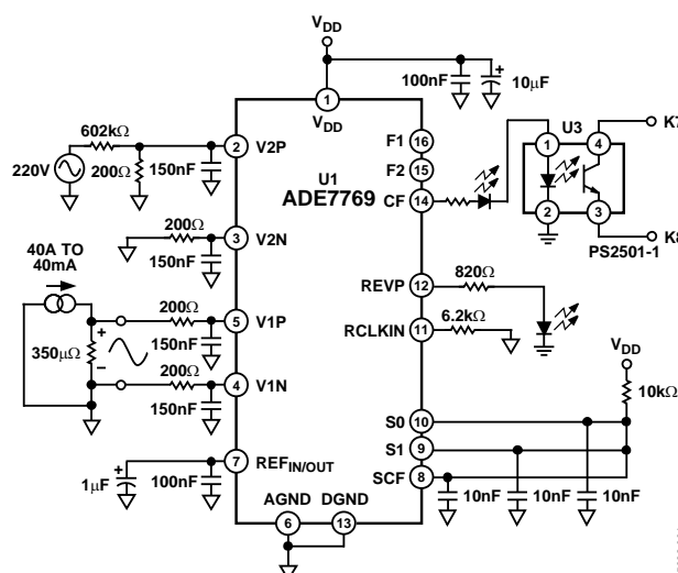
Figure 4. Test Circuit for Performance Curves
