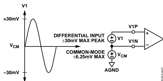
Figure 17. Maximum Signal Levels, Channel V1
