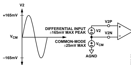
Figure 18. Maximum Signal Levels, Channel V2
