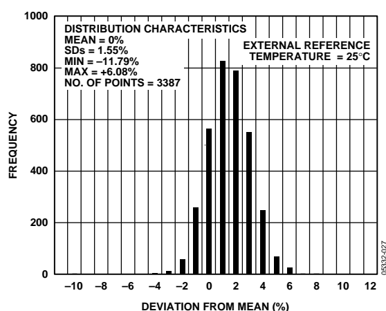
Figure 14. Part-to-Part CF Deviation from Mean
