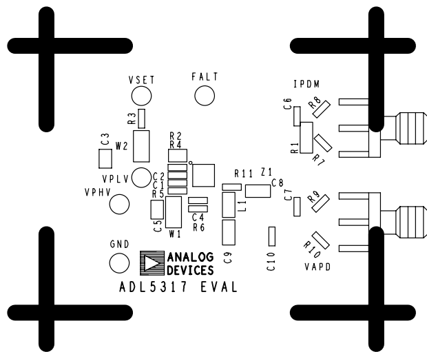
Figure 32. ADL5317 Evaluation Board Silkscreen
