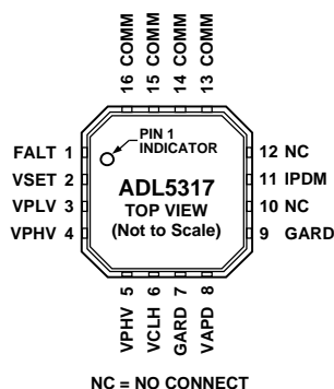
Figure 2. Pin Configuration
