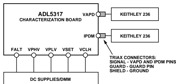
Figure 25. Primary Characterization Setup
