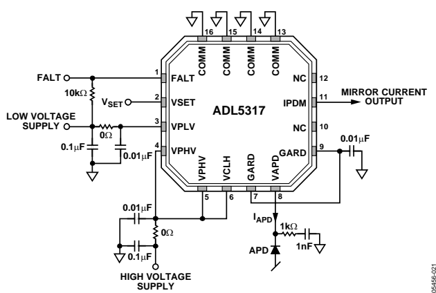
Figure 19. Basic Connections
