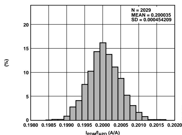
Figure 18. Distribution of I_{PDM}/I_{APD} at V_{PHV} = 60 V, V_{SET} = 1.0 V, I_{APD} = 50 \mu A
