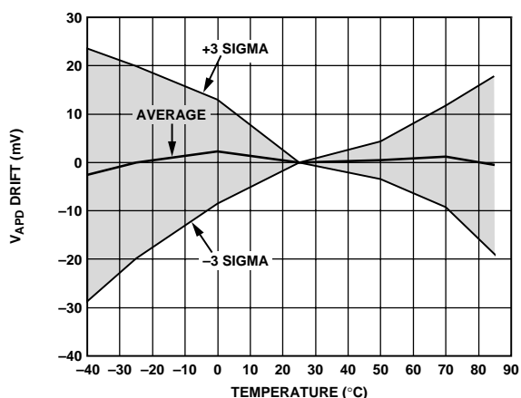
Figure 11. Temperature Drift of V_{APDr} , 3\sigma to Either Side of Mean
