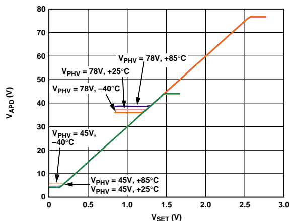
Figure 4. V_{APD} vs. V_{SET} for Multiple Temperatures, V_{PHV} = 78\text{ V} and V_{PHV} = 45\text{ V} , I_{APD} = 5\text{ }\mu\text{A}
