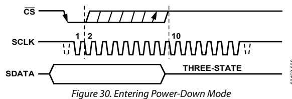
Figure 30. Entering Power-Down Mode
