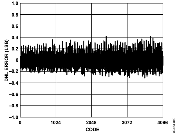
Figure 10. Typical DNL for the AD7451 for V_{\text{DD}} = 5 \text{ V}
