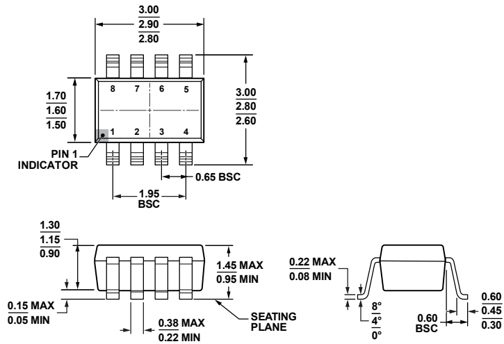
COMPLIANT TO JEDEC STANDARDS MO-178-BA Figure 36. 8-Lead Small Outline Transistor Package [SOT-23] (RJ-8) Dimensions shown in millimeters
