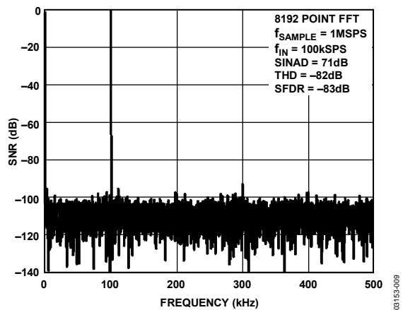
Figure 9. AD7451 Dynamic Performance for V_{\text{DD}} = 5 \text{ V}
