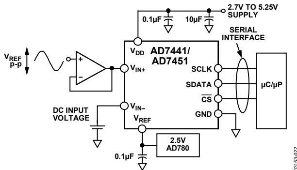
Figure 22. Typical Connection Diagram
