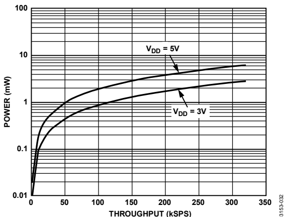
Figure 32. Power vs. Throughput Rate for Power-Down Mode
