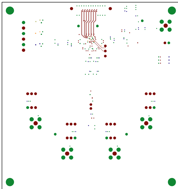
Figure 46. Evaluation Board Layout, Secondary Side
