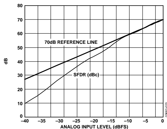
Figure 20. Two-Tone SFDR vs. Analog Input Level with f_{\text{IN1}} = 15 \text{ MHz} and f_{\text{IN2}} = 16 \text{ MHz} , f_{\text{SAMPLE}} = 65 \text{ MSPS}
