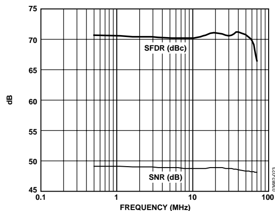
Figure 18. SNR/SFDR vs. f_{\text{IN}} , f_{\text{SAMPLE}} = 65 \text{ MHz}
