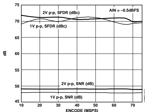
Figure 12. SNR/SFDR vs. f_{SAMPLE} , f_{IN} = 2.4 MHz
