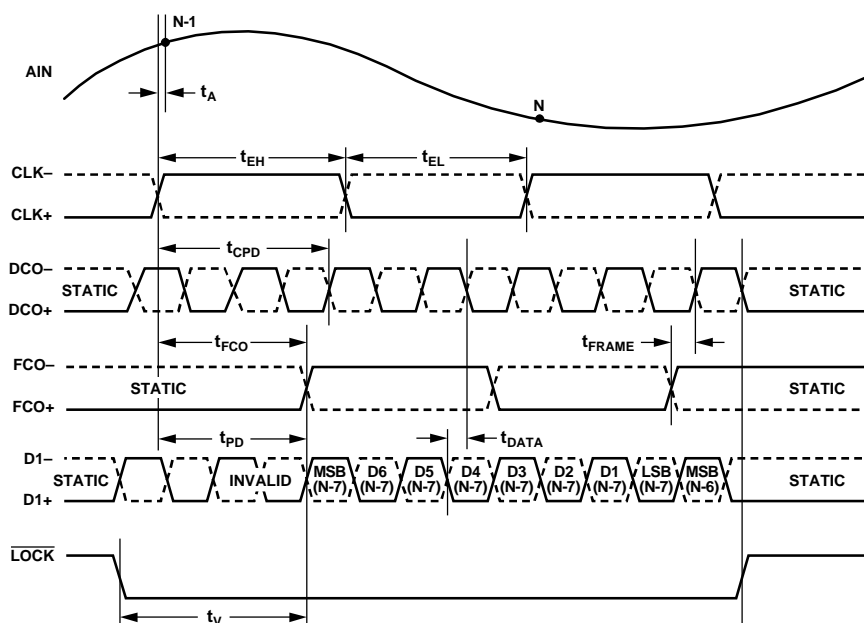
Figure 2. Timing Diagram
