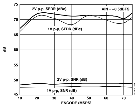
Figure 14. SNR/SFDR vs. f_{SAMPLE} , f_{IN} = 35 MHz
