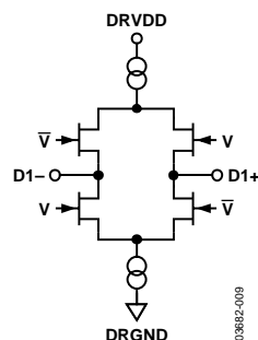
Figure 7. Equivalent Digital Output Circuit
