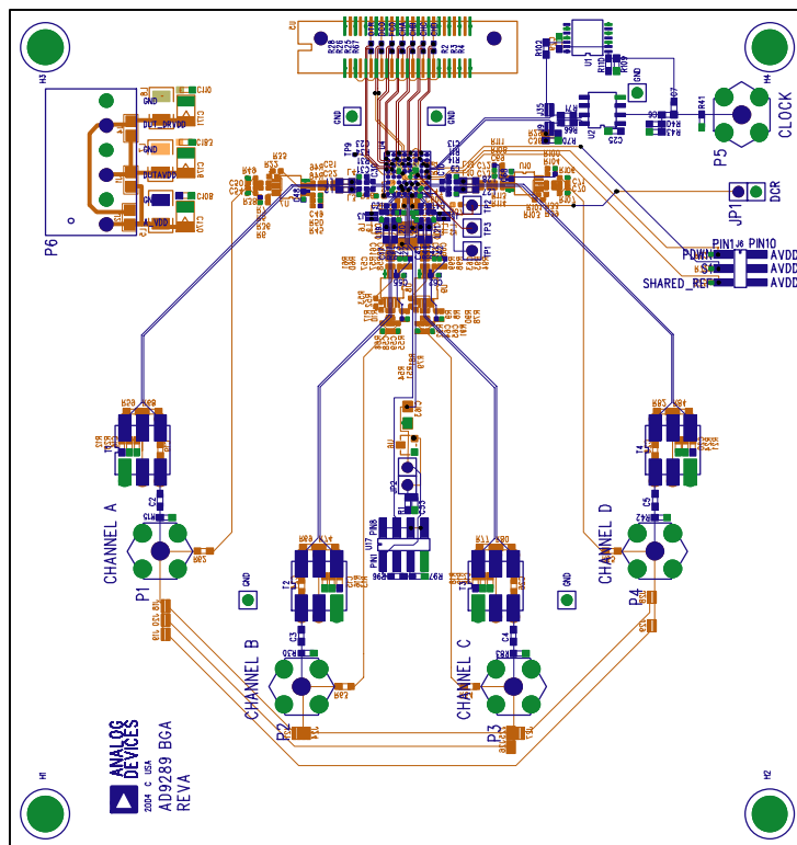
Figure 42. Evaluation Board Layout, Primary Side
