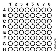
Figure 3. BGA Top View (Looking Through)
