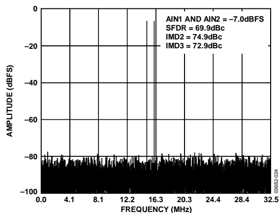
Figure 19. Two-Tone 32k FFT with f_{\text{IN1}} = 15 \text{ MHz} and f_{\text{IN2}} = 16 \text{ MHz} , f_{\text{SAMPLE}} = 65 \text{ MSPS}
