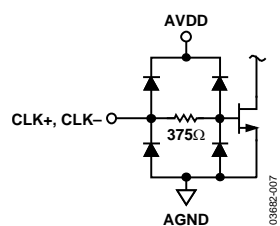
Figure 5. Equivalent Clock Input Circuit
