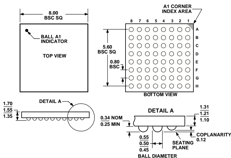
Figure 48. 64-Lead Chip Scale Package Ball Grid Array [CSP_BGA] (BC-64-1)
