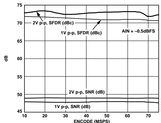
Figure 13. SNR/SFDR vs. f_{SAMPLE} , f_{IN} = 10.3 MHz
