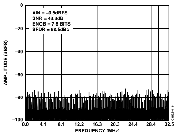
Figure 11. Single-Tone 32k FFT With f_{IN} = 35 MHz, f_{SAMPLE} = 65 MSPS
