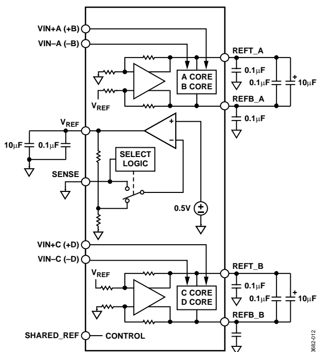
Figure 33. Internal Reference Configuration
