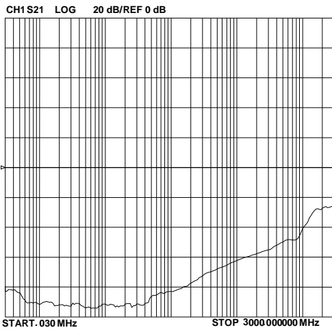
Analog Crosstalk
