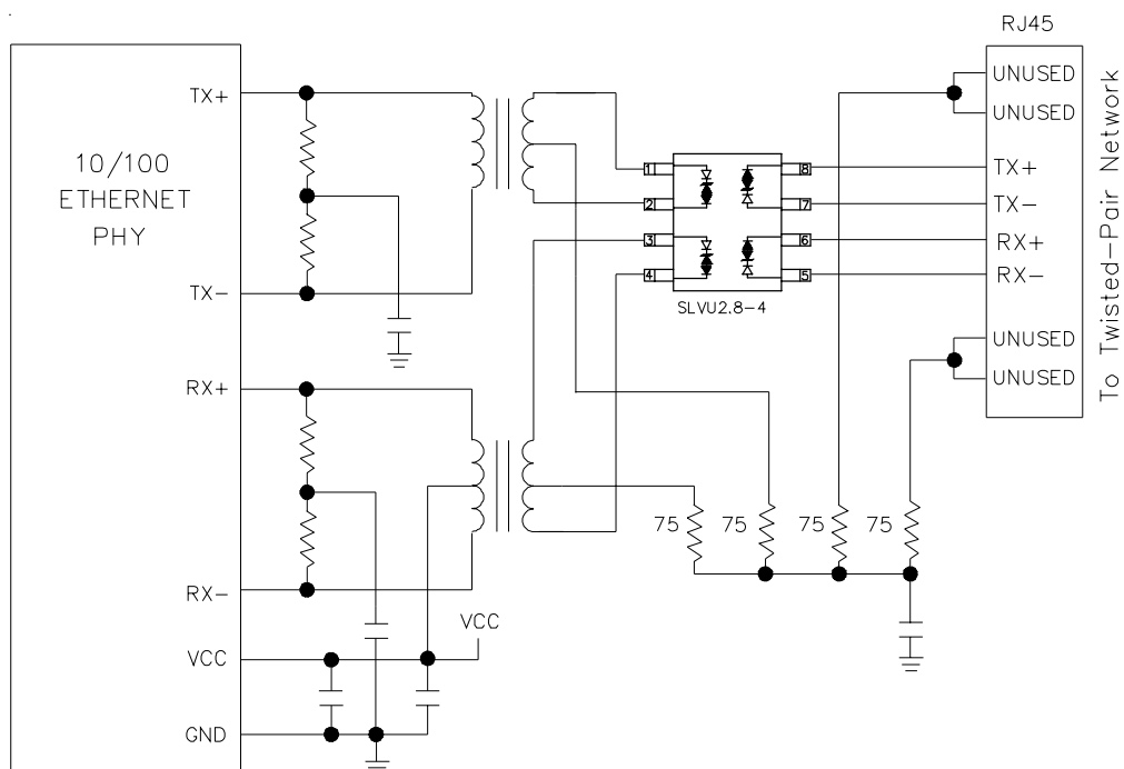
10/100 Ethernet Protection Circuit
